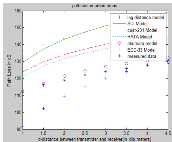
Figure 1: Comparative analysis of different path loss models.
