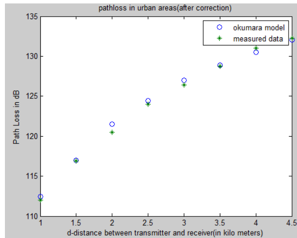
Figure 3: Okumara model and Field measured data (After correction factor).
