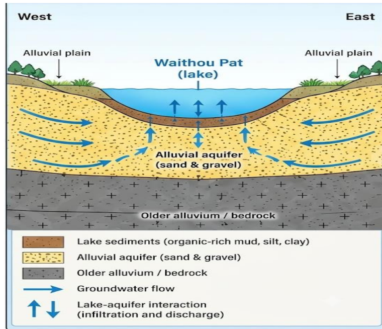
Figure 3. Conceptual geological and hydrogeological cross-section of Waithou Pat illustrating the lake basin, shallow lake sediments, underlying alluvial materials and possible groundwater-flow pathways. Arrows indicate hypothesised lake–aquifer exchange; the section is interpretive and is not based on site-specific groundwater-head measurements.
