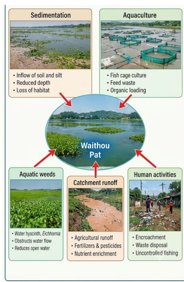
Figure 7. Conceptual summary of major environmental pressures affecting Waithou Pat, including catchment erosion and sedimentation, aquaculture-related inputs, excessive aquatic-weed growth, runoff and other human activities. The arrows indicate plausible pathways through which these pressures may interact and affect water quality and wetland habitat.
