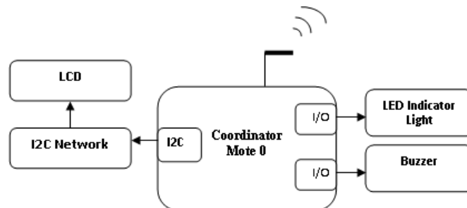
Fig – 3 Coordinate mote system
