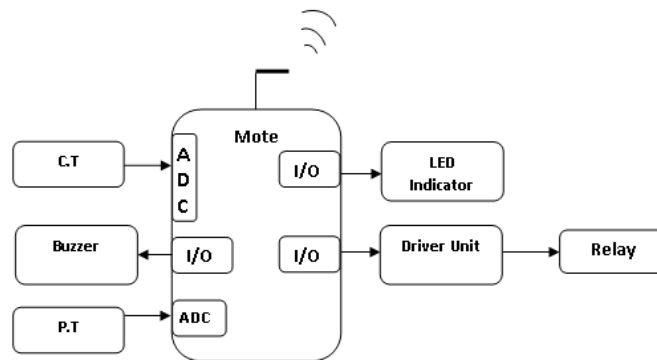
Fig – 2 Reference mote system
