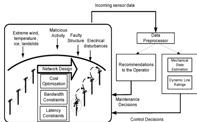
Fig – 1 Framework of sensor network
