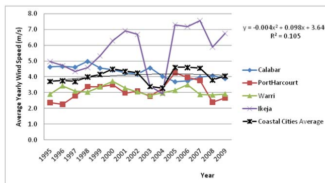
Fig 4a: Trend showing Annual average wind speed (m/s) for Coastal cities against year
