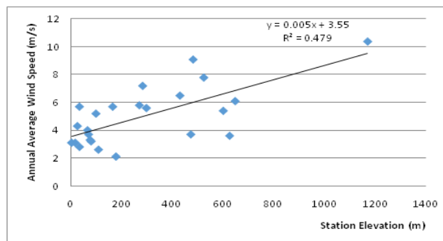
Fig 2: Annual average wind speed (m/s) against Station elevation (m)
