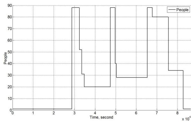
Fig. 1.1.3. Visitors' schedule
