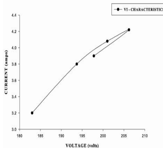
Figure 4: VI Characteristics
