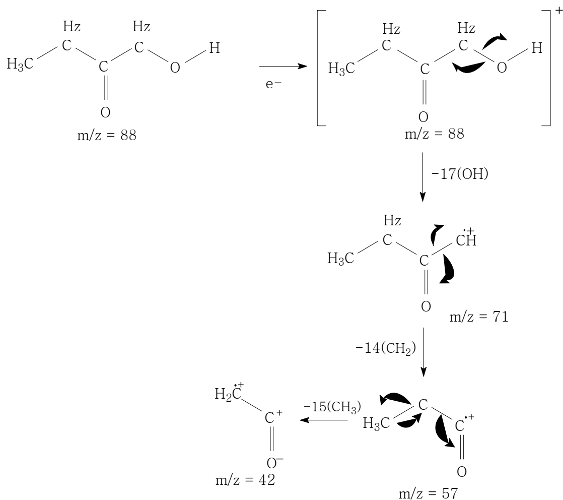
Figure 2. Prediction of compound fragmentation pattern peak 6 or 1 hydroxy 2 butanone.
