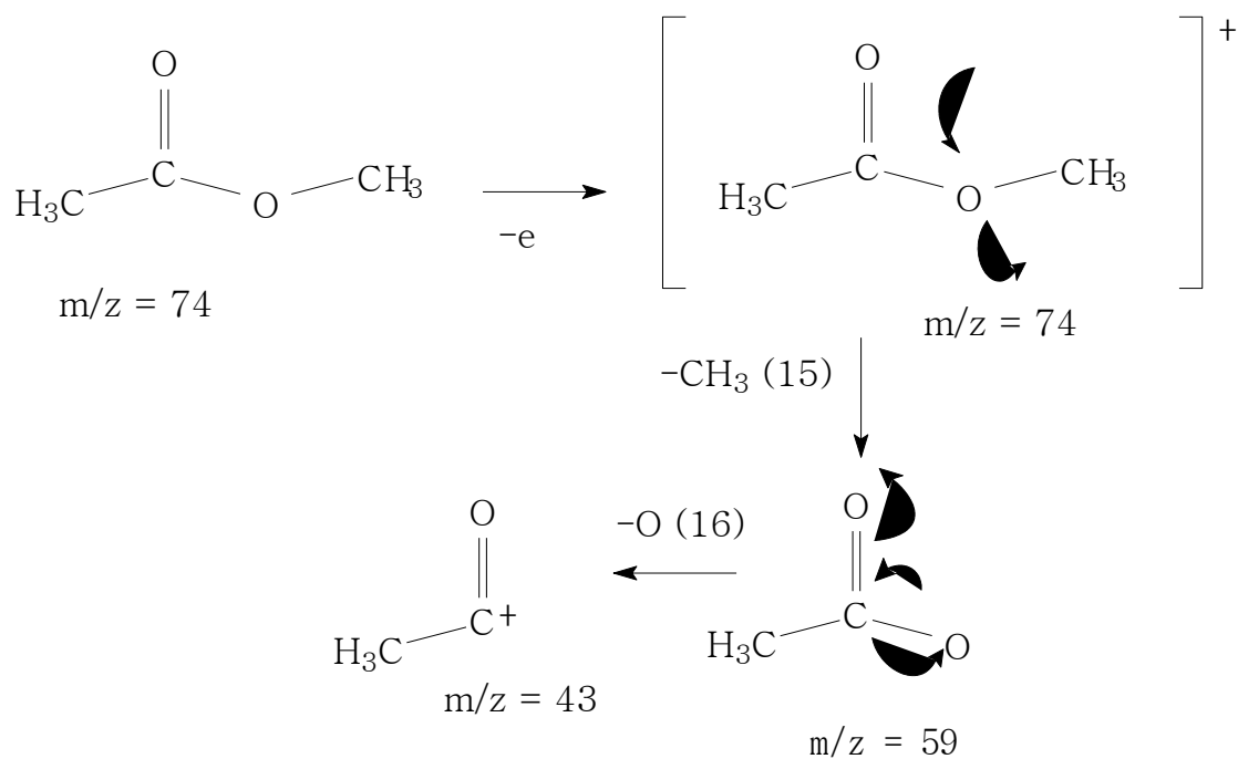
Figure 1. Prediction of ion release fragmentation pattern or peak 3 compound molecule or methyl acetate.
