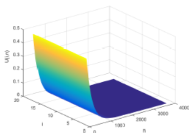
FIGURE 7 – Evolution of the discrete solution, source f(U) = (U_i^{(n)})^{-p} , \varepsilon = 0 , \varphi_i = \frac{0.99 + \varepsilon \sin(\pi x)}{2} , I = 32 (implicit scheme).
