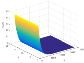
FIGURE 1 – Evolution of the discrete solution, source f(U) = (U_i^{(n)})^{-p} , \varepsilon = 1/10000 , \varphi_i = \frac{0.99+\varepsilon \sin(\pi x)}{2} , I = 16 (implicit scheme).
