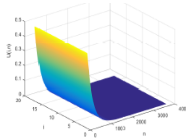
FIGURE 5 – Evolution of the discrete solution, source f(U) = (U_i^{(n)})^{-p} , \varepsilon = 0 , \varphi_i = \frac{0.99+\varepsilon \sin(\pi x)}{2} , I = 16 (implicit scheme).
