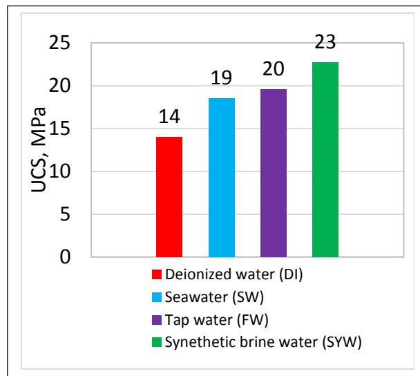
Figure 7b: Uniaxial compressive strength DI, FW, SW and SYW plugs
