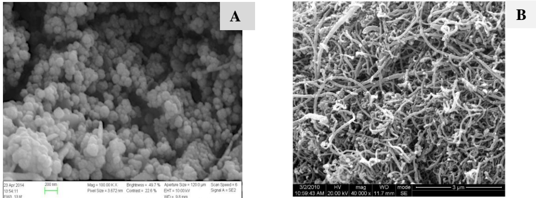
Figure 4: Scanning electron microscopic (SEM) of (A) Silica; (B) MWCNT
