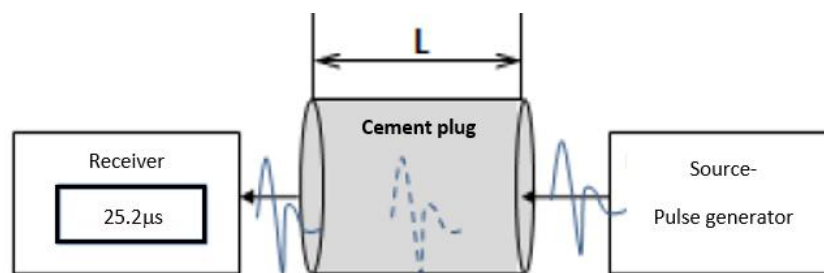
Figure 1: Sonic wave propagation through core plug
