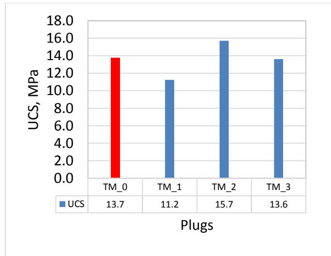
Figure 10: Effect of MWCNT-SiO 2 composite on cement
