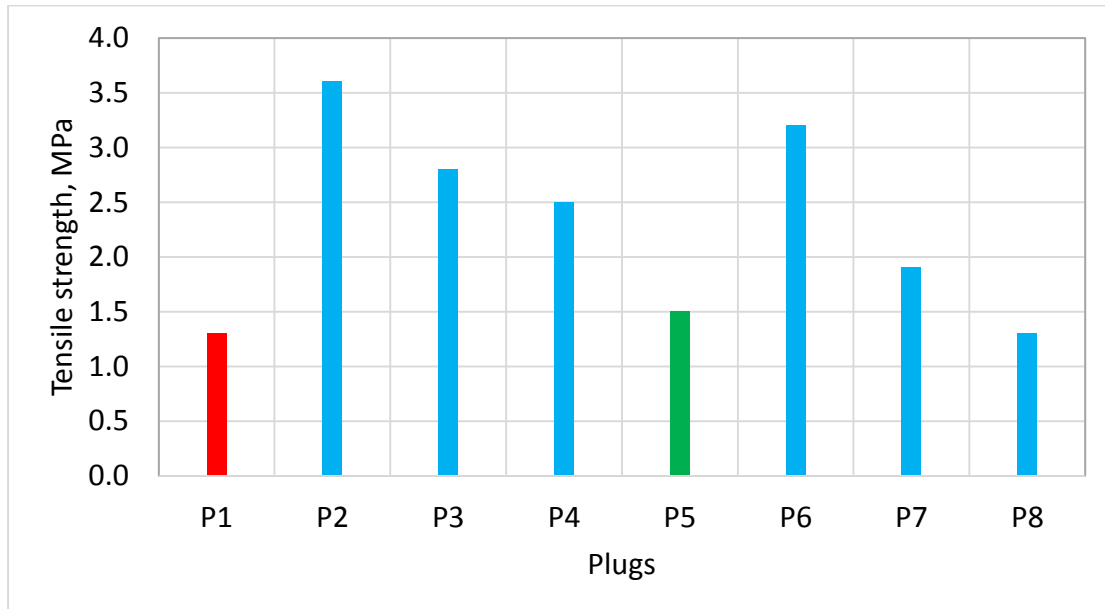
Figure 9: Effect of SiO 2 concentration and salinity on tensile test [33]
