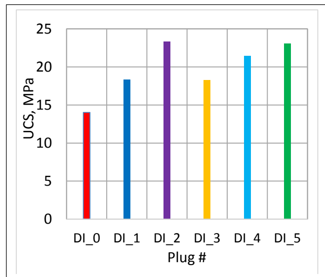
Figure 6b: Uniaxial compressive strength DI based plugs
