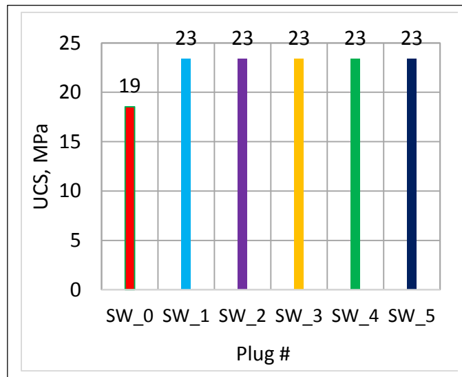
Figure 5b: Uniaxial compressive strength SW based plugs
