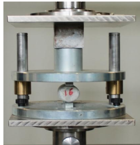
Figure 3: Brazilian test setup
