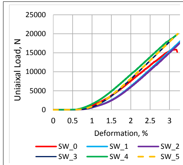
Figure 5a: Uniaxial compressive load on SW based plugs
