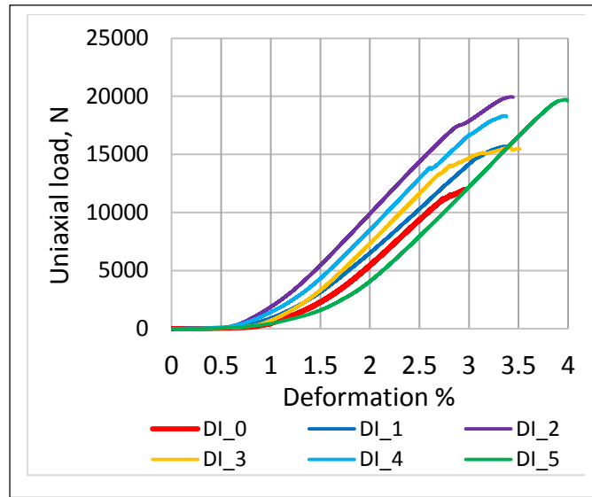
Figure 6a: Uniaxial compressive load on DI based plugs
