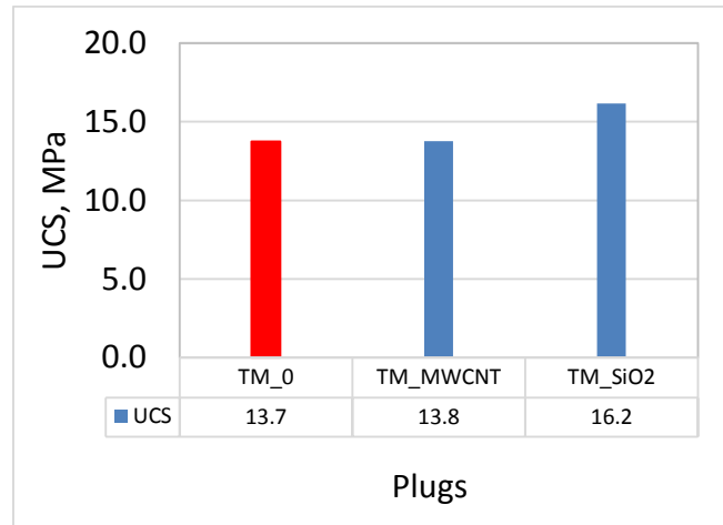
Figure 11: Effect of single MWCNT and SiO 2 on cement
