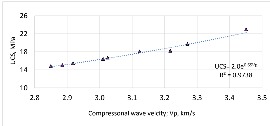
Figure 13: New UCS- V_p empirical model
