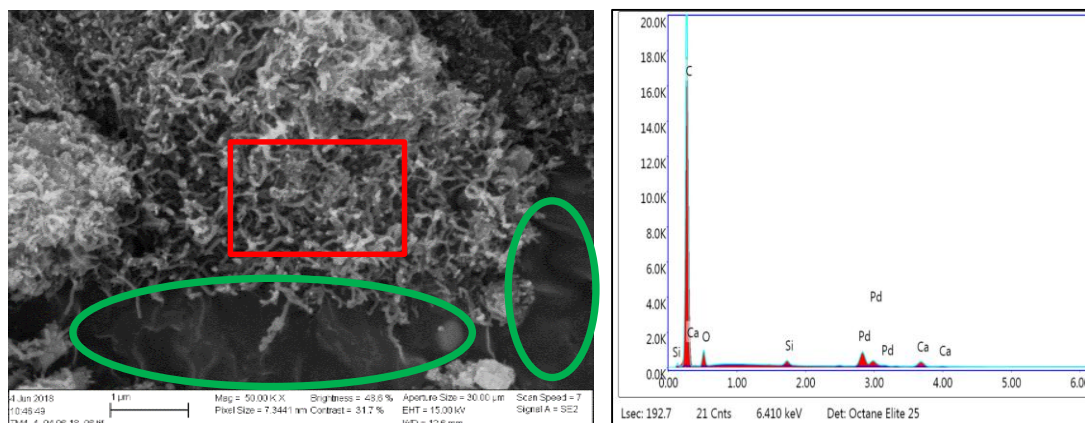
Figure 12a: SEM Picture sporting at MWCNT Figure 12b: EDS-analysis of the MWCNT
