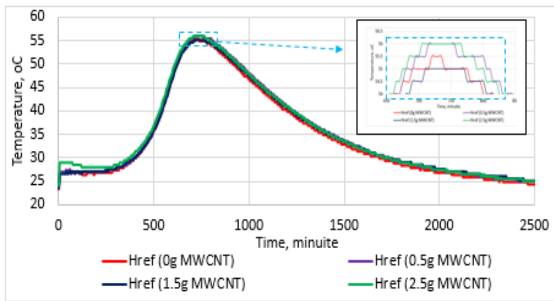
Figure 8: Heat of hydration
