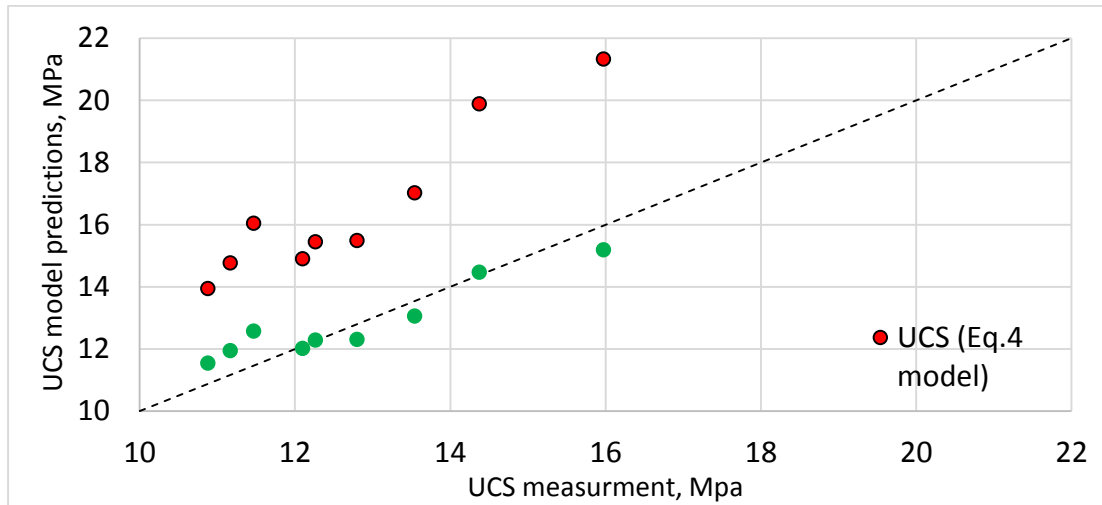
Figure 14: Comparison between model prediction (Eq.4, Eq.5) and measurement
