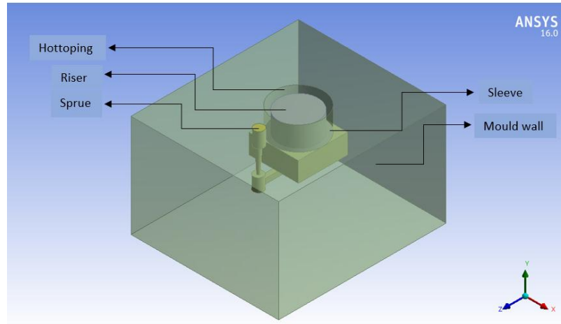
Figure 1: Casting with sand mould
