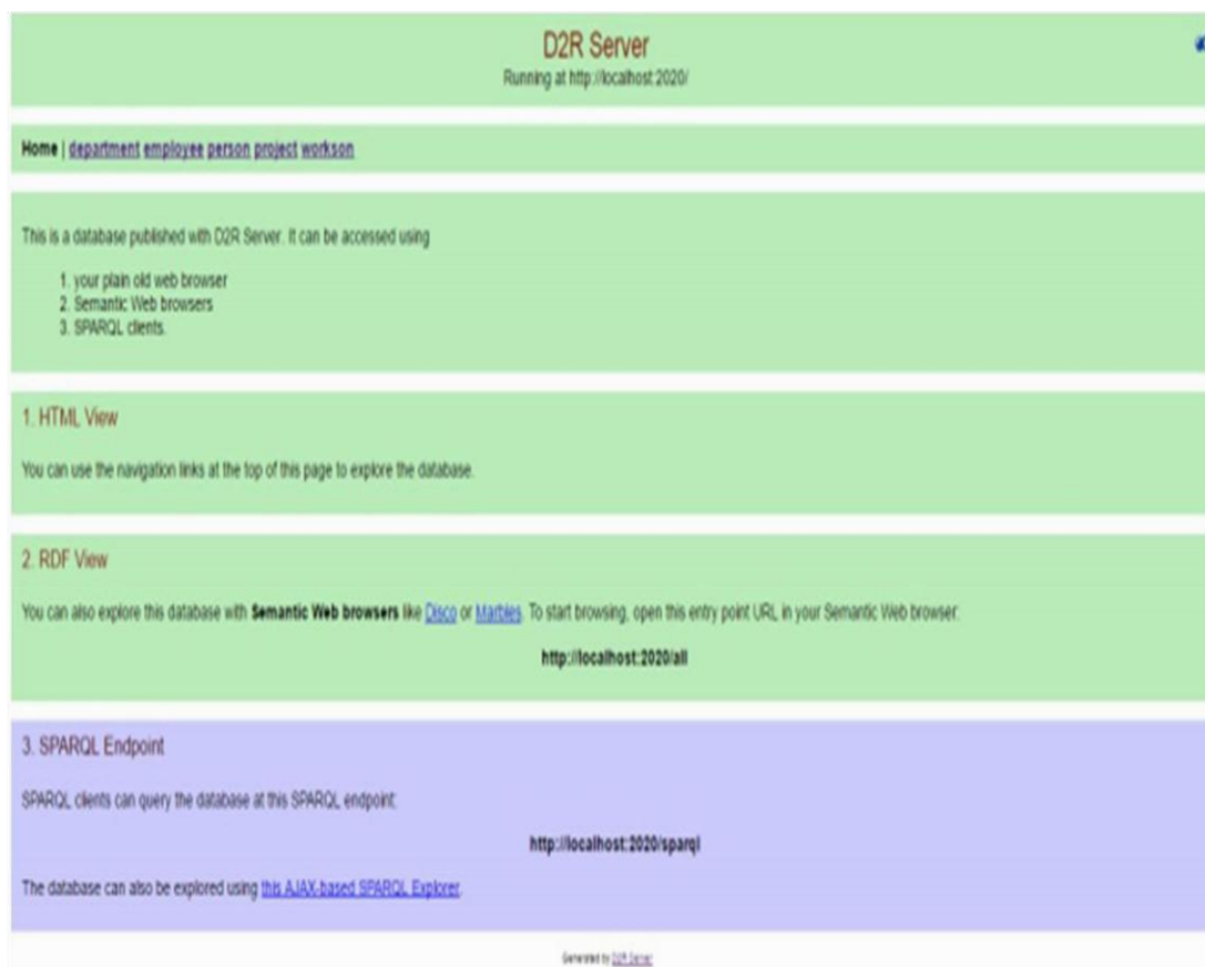
Fig.11 Publishing file generated by D2RQ on D2R-Server
