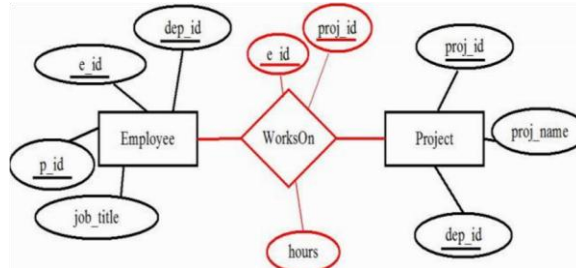
Fig.8 Many-to-many relationship
