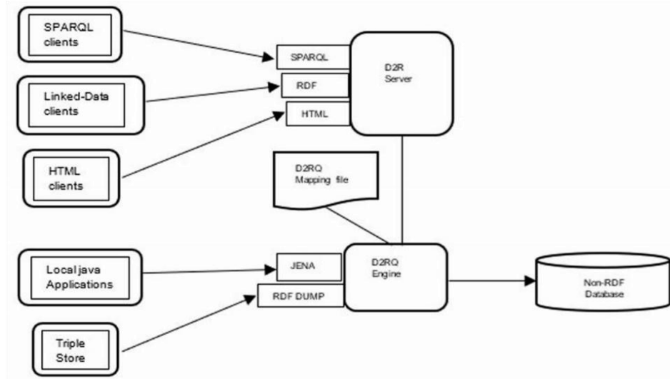
Fig 1. Functional Component of D2RQ platform
