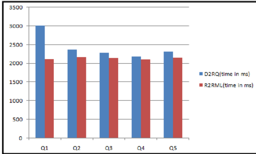
Fig 14. Time Analysis Graph
