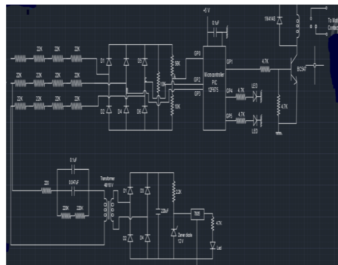
Fig.2. Autostart Circuit
