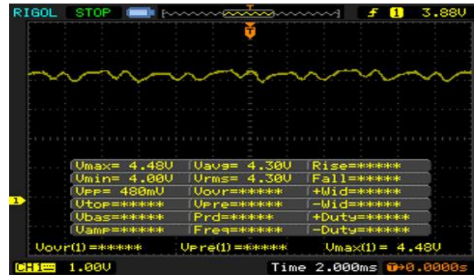
Fig.7. Waveform at point A
