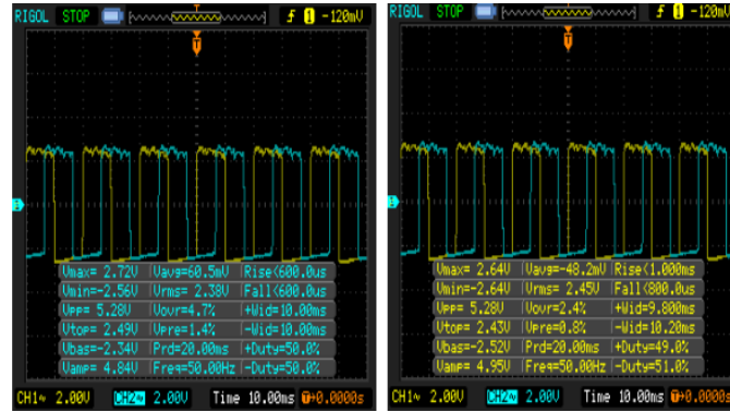
Fig.9. Waveforms at point B and C
