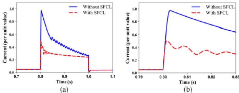
Fig. 8. (a) Short circuit current curves with and without SFCL. (b) Rising edge of short circuit current curves with and without SFCL.
