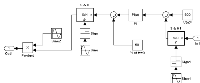
Fig 3. Simulink Diagram for DC link voltage control and generation of current reference.
