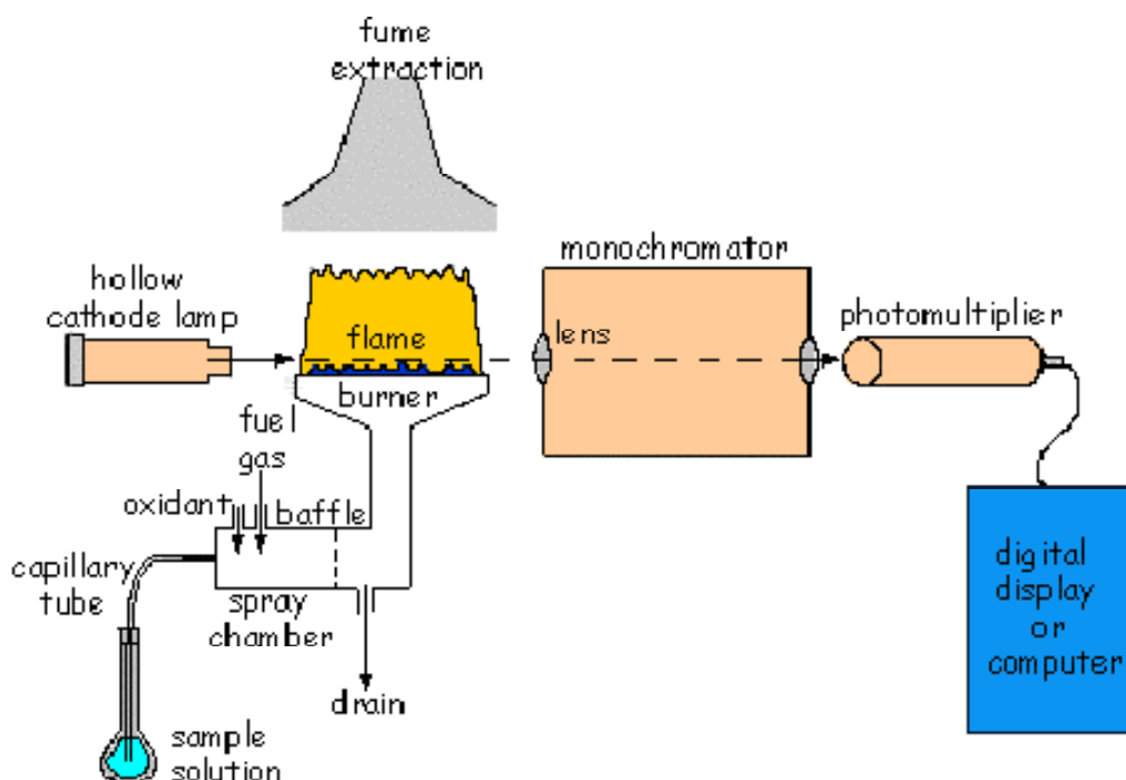
Figure 1: A schematic diagram of atomic absorption spectrometer
