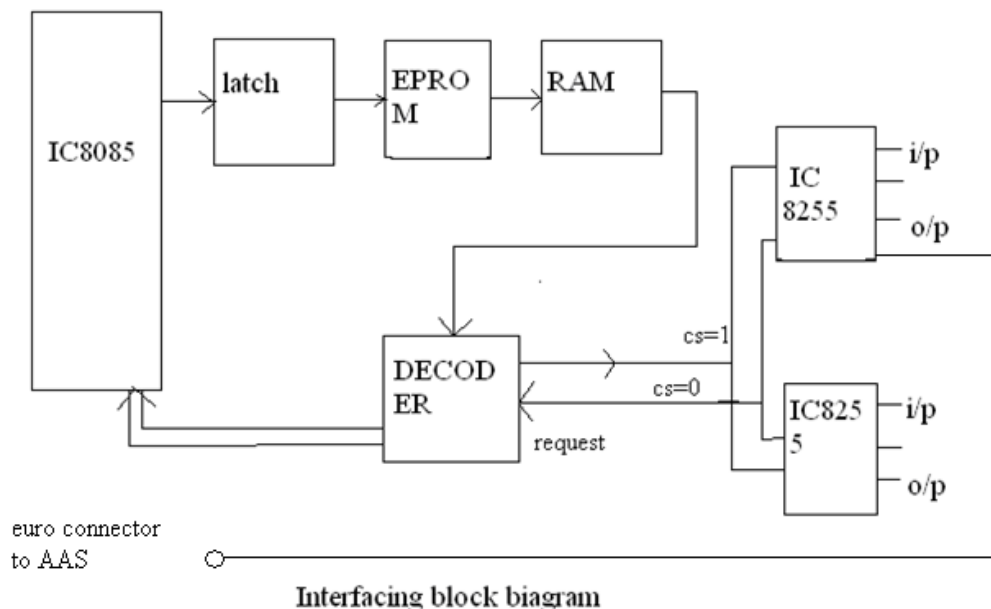
Figure 2: Block diagram of interfacing ASS and AGC
