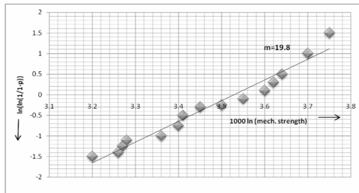
Figure 7: Results of the Weibull's statistics for mechanical strength (MPa) of the fired A-samples.
