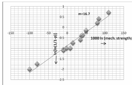
Figure 6: Results of the Weibull's statistics for mechanical strength (MPa) of the green A-samples.
