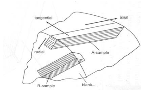
Figure 1: Samples and directions of the texture. Dashed lines indicate orientation of the platelike kaolinite crystals.
