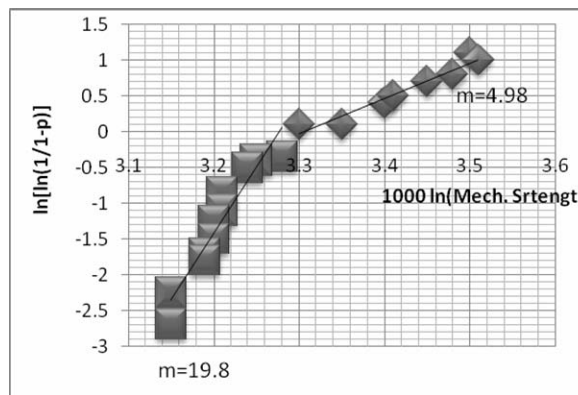
Figure 5: Result of the weibull's statistics for mechanical strength (Mpa) of the fired R-samples.
