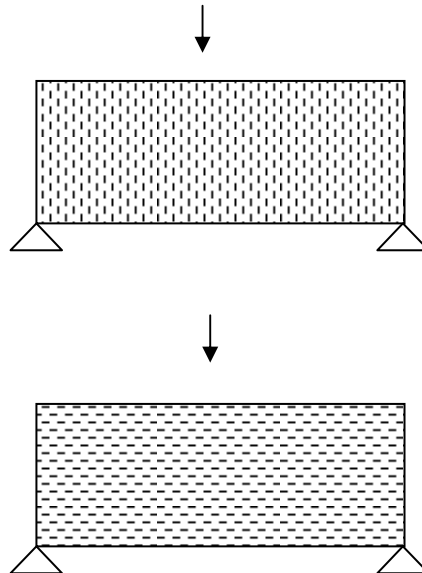
Figure 3: Three –point bending the R-samples with radial texture (upper picture) and A- samples with axial texture (lower picture). Dashed lines indicate positioning of the platelike kaolinite crystals.
