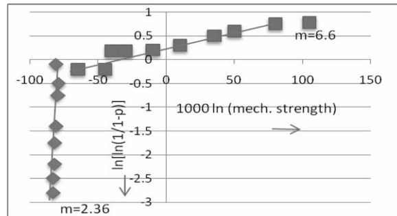
Figure 4: Result of the weibull's statistics for mechanical strength (Mpa) of the green R-samples. Weibull's moduli are written beside the liner approximations.
