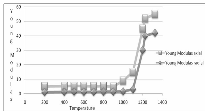
Figure 2: Dependence of the Young' modulus on firing temperature.
