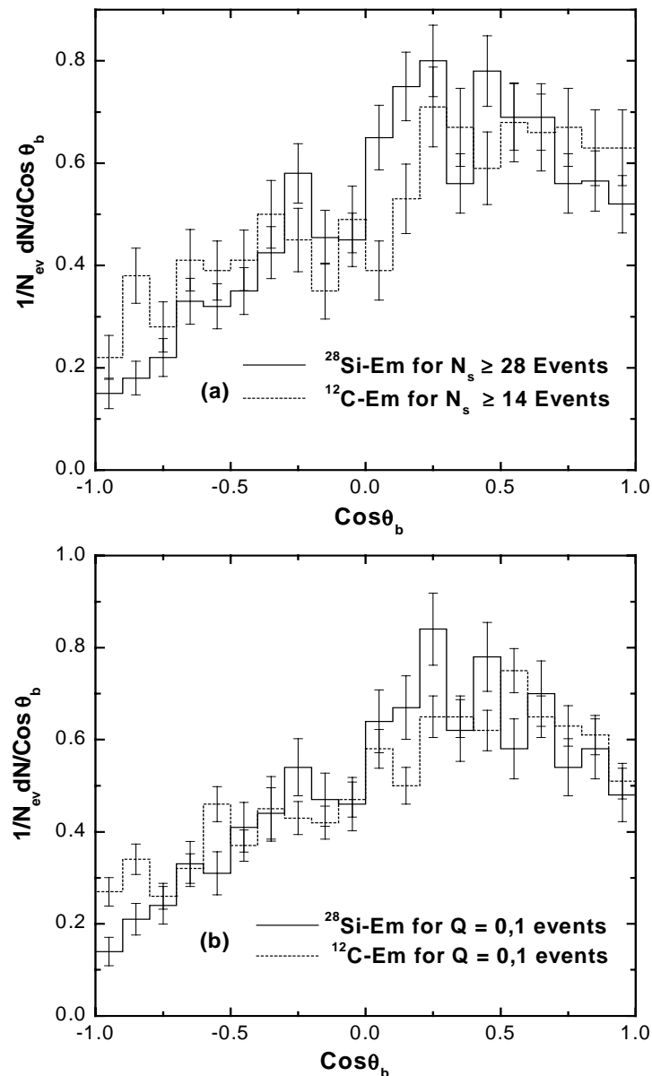
Figure 6: Angular distributions of black tracks for ^{28}\text{Si-Em} and ^{12}\text{C-Em} interactions at 4.5A GeV/c (a) for N_s \geq 28 and N_s \geq 14 events (b) for Q = 0,1 events.
