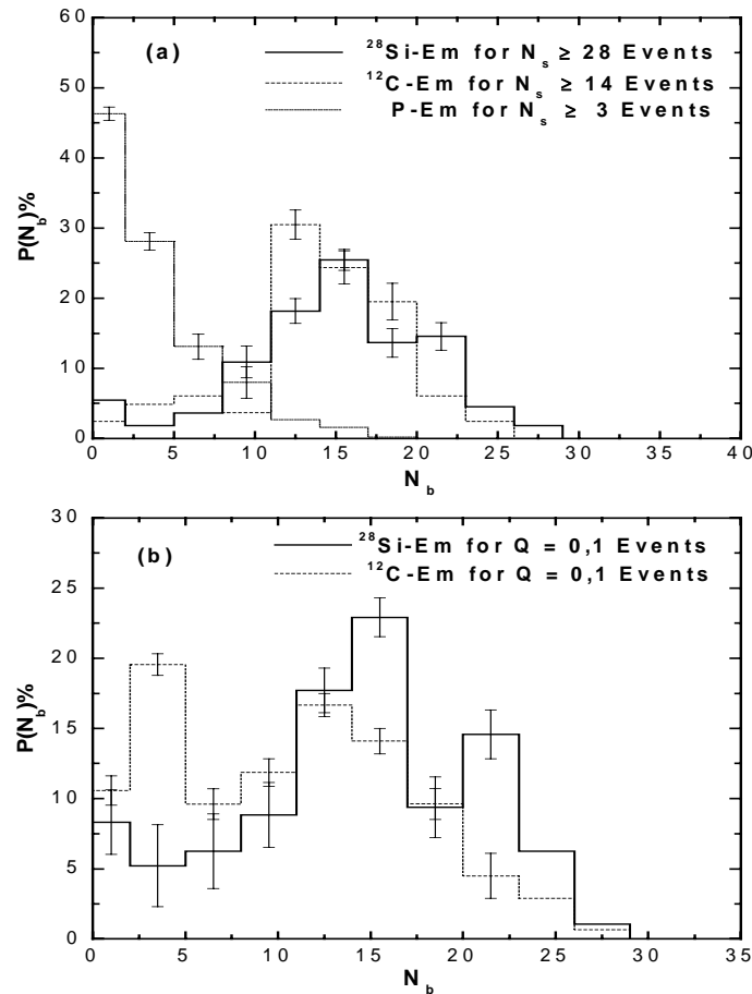
Figure 2: Multiplicity distributions of black tracks (a) for N_s \geq 28 events of ^{28}\text{Si-Em} , N_s \geq 14 events of ^{12}\text{C-Em} and N_s \geq 3 events of P-Em (b) for Q = 0,1 ensembles of ^{28}\text{Si-Em} and ^{12}\text{C-Em} interactions at 4.5A GeV/c.
