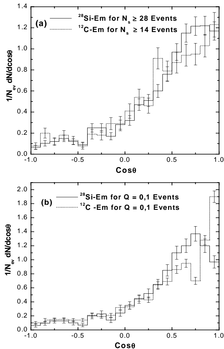
Figure 5: Angular distributions of grey tracks for ^{28}\text{Si-Em} and ^{12}\text{C-Em} interactions at 4.5A GeV/c (a) for N_s \geq 28 and N_s \geq 14 events (b) for Q = 0,1 events.
