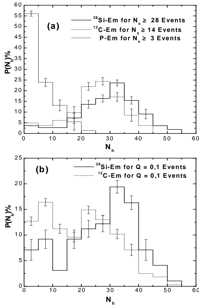
Figure 3: Multiplicity distributions of heavily ionizing tracks (a) for N_s \geq 28 events of ^{28}\text{Si-Em} , N_s \geq 14 events of ^{12}\text{C-Em} and N_s \geq 3 events of P-Em (b) for Q = 0,1 ensembles of ^{28}\text{Si-Em} and ^{12}\text{C-Em} interactions at 4.5A GeV/c.
