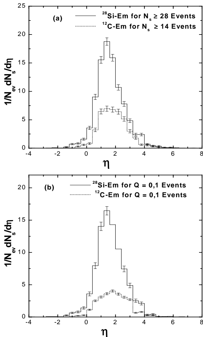
Figure 7: Pseudorapidity distributions of shower particles for ^{28}\text{Si} -Em and ^{12}\text{C} -Em interactions at 4.5A GeV/c (a) for N_s \geq 28 and N_s \geq 14 events (b) for Q = 0,1 events.
