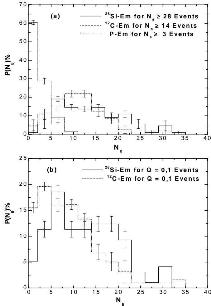
Figure 1: Multiplicity distributions of grey tracks (a) for N_s \geq 28 events of ^{28}\text{Si} -Em, N_s \geq 14 events of ^{12}\text{C} -Em and N_s \geq 3 events of P-Em (b) for Q = 0,1 ensembles of ^{28}\text{Si} -Em and ^{12}\text{C} -Em interactions at 4.5A GeV/c.
