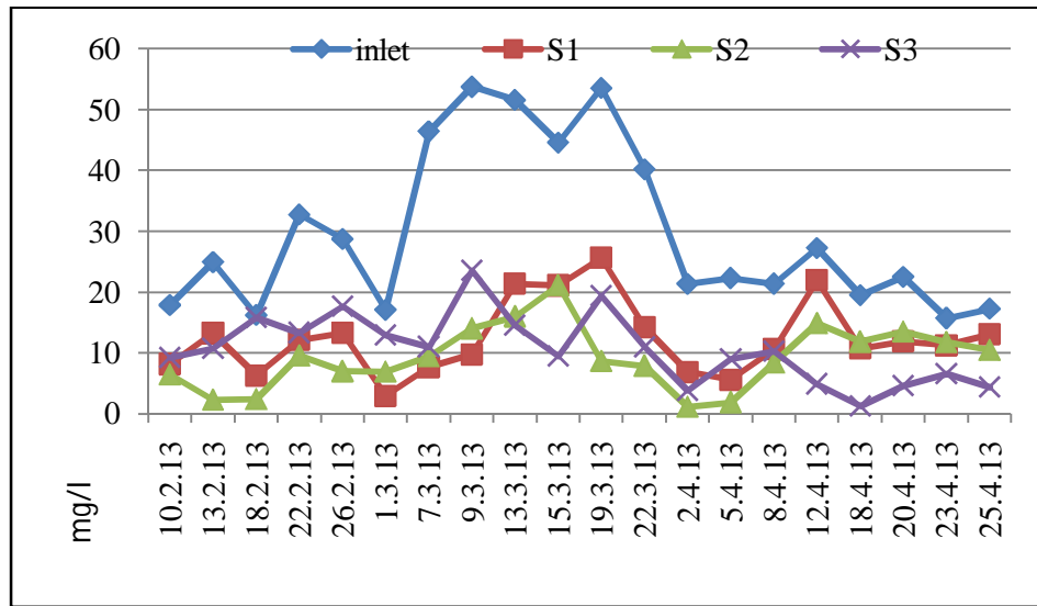
Graph 1: Comparison for NH 4 -N removal.
