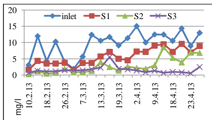
Graph 4: Comparison for phosphorus removal.
