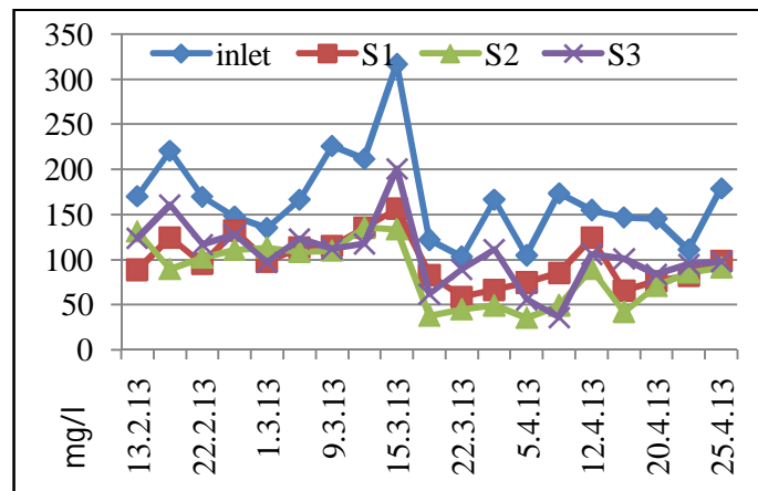
Graph 6: Comparison for COD removal.
