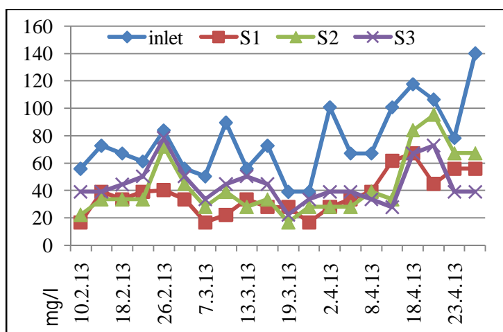
Graph 3: Comparison for TKN removal.
