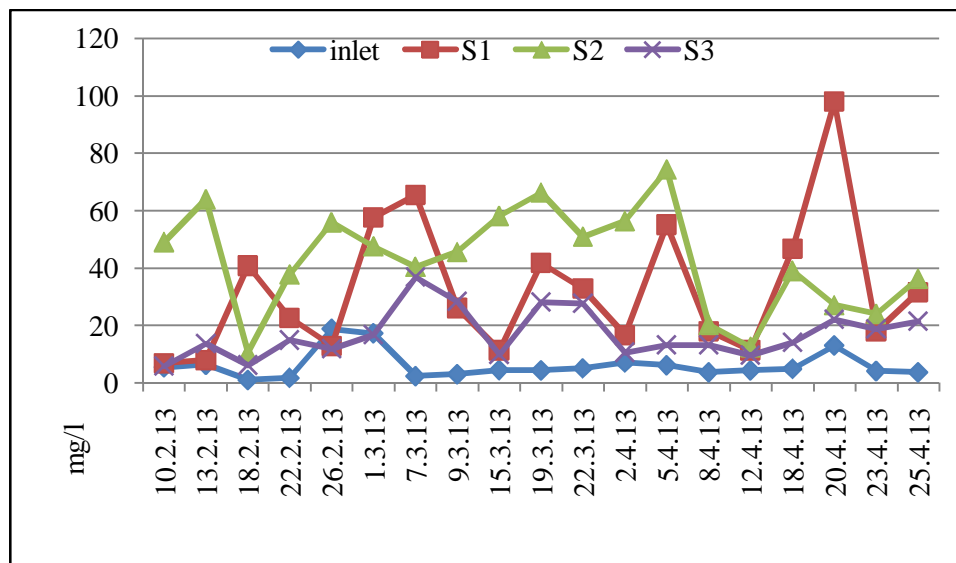
Graph 2: Comparison for NO 3 -N removal.
