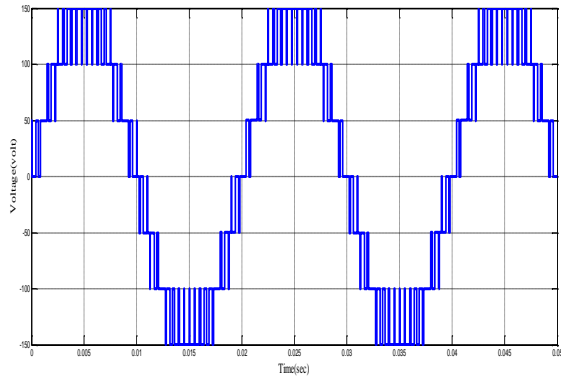
Fig .7: Output voltage waveform of 7-level Fibonacci Series MLI
