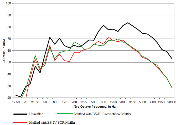
Figure 5.a. Exhaust spectrums for Idling condition
