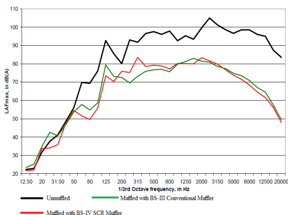
Figure 5.c. Exhaust spectrums for Fly-up condition
