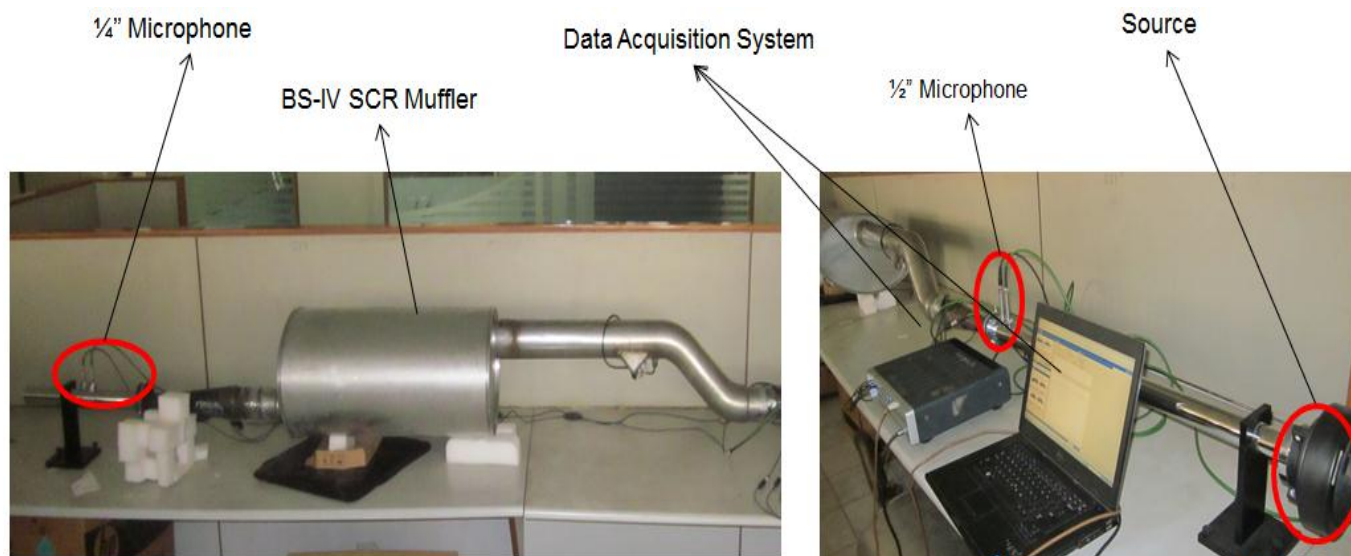
Figure 2. Transmission Loss Test Setup
