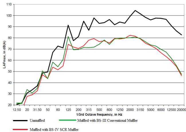
Figure 5.b. Exhaust spectrums for Max. Power condition
