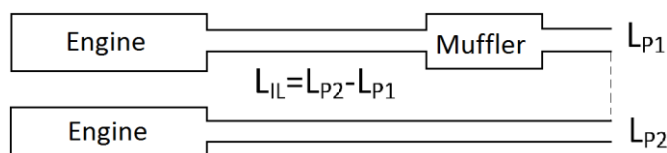
Figure 3. Insertion Loss Definition
