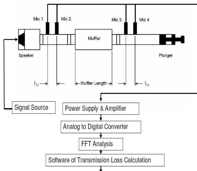
Figure 1. Flow diagram of experimental set up to measure TL of mufflers
