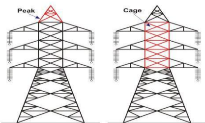
Fig.5. Cage in a transmission tower
