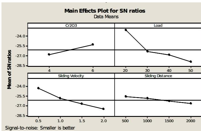
Figure 5. ANOVA Analysis
