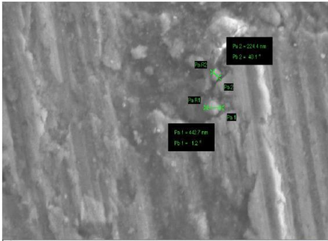
Figure 4. SEM image of Specimen 2
