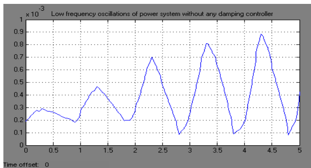
Figure 13. Rotor speed Vs time, LLLG fault at G4 without IPFC
