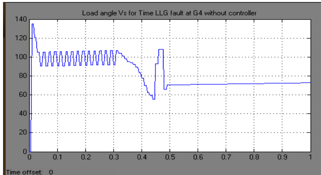
Figure 7. Load angle Vs time, LLG fault at G4 without controller
