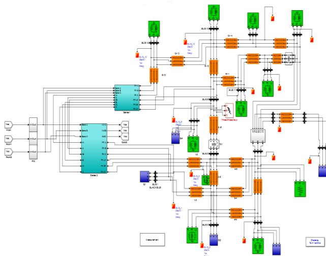
Figure 3. MATLAB/SIMULINK diagram of IEEE 14 bus system using IPFC with fault.
