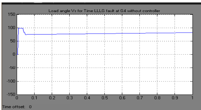
Figure 8. Load angle Vs time, LLLG fault at G4 without controller
