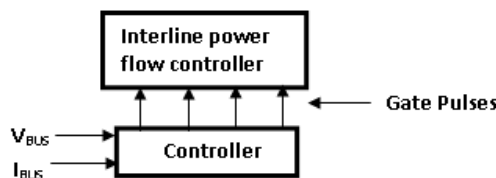
Figure 2. Controller structure with IPFC.
