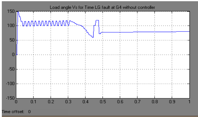
Figure 6. Load angle Vs time, LG fault at G4 without controller
