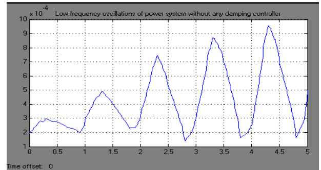
Figure 14. Rotor speed Vs time, LLLG fault at G4 without IPFC
