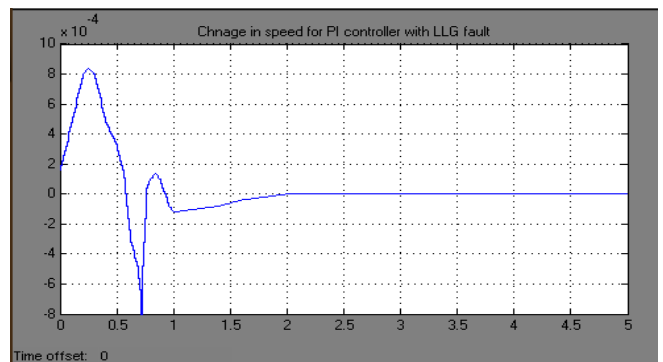
Figure 16. Rotor Speed Vs time, LLLG fault at G4 with IPFC using PI Controller
