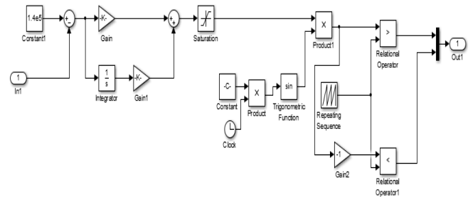
Figure 5. MATLAB/SIMULINK diagram of PI controller.
