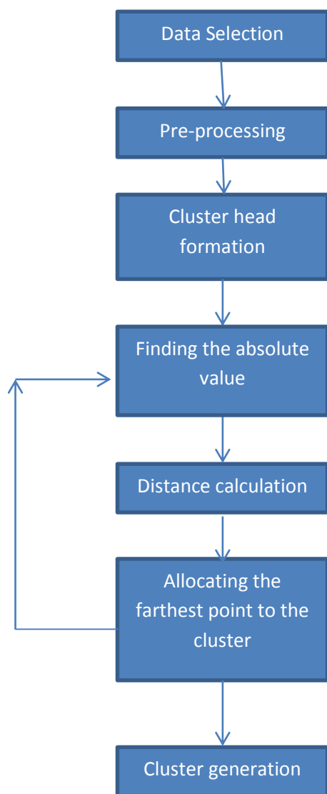
Figure 3. Architecture Diagram
