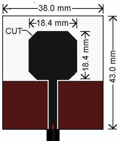
Figure 4: Structure of Modified RMSA with Straight Edge Cut (Type B)
