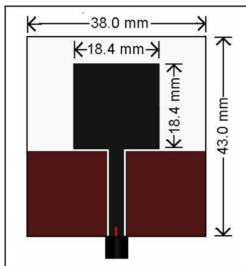
Figure 1. Structure of Basic Rectangular Microstrip Patch Antenna (Type A)
