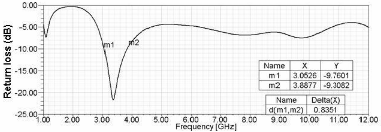
Figure 2. Return Loss vs. Frequency for simple RMSA (Type A)
