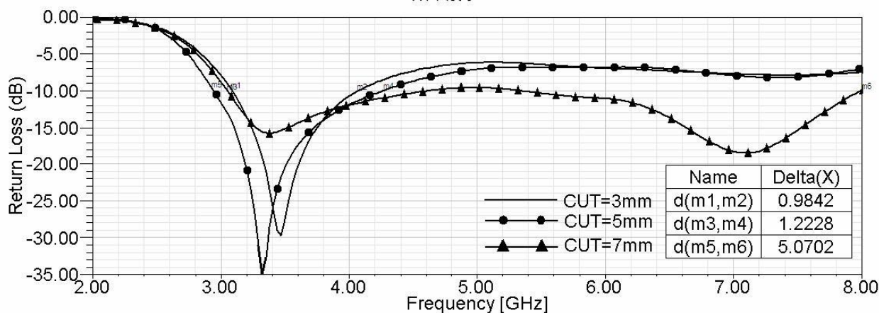
Figure 5. Return Loss vs. Frequency for modified RMSA with straight edge cut
