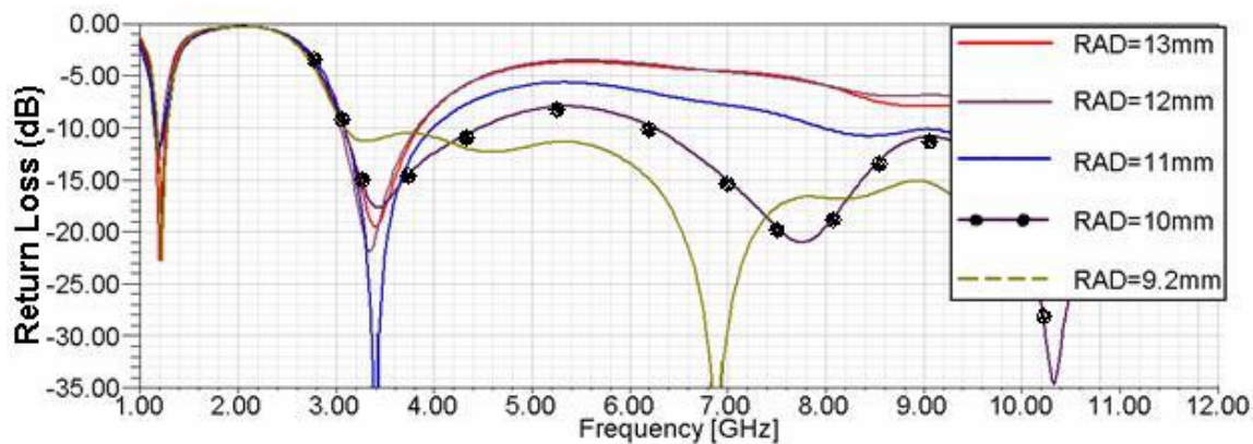
Figure 8. Return Loss vs. Frequency for modified RMSA with circular edge cut
