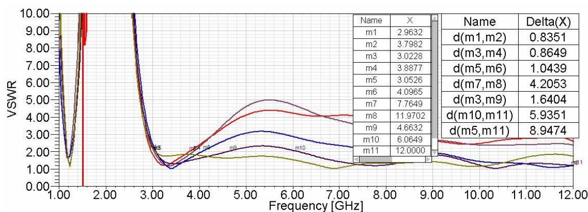
Figure 9. VSWR vs. Frequency for modified RMSA with circular edge cut
