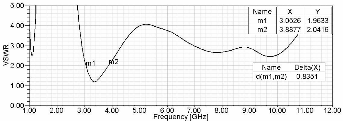
Figure 3. VSWR vs. Frequency for simple RMSA (Type A)
