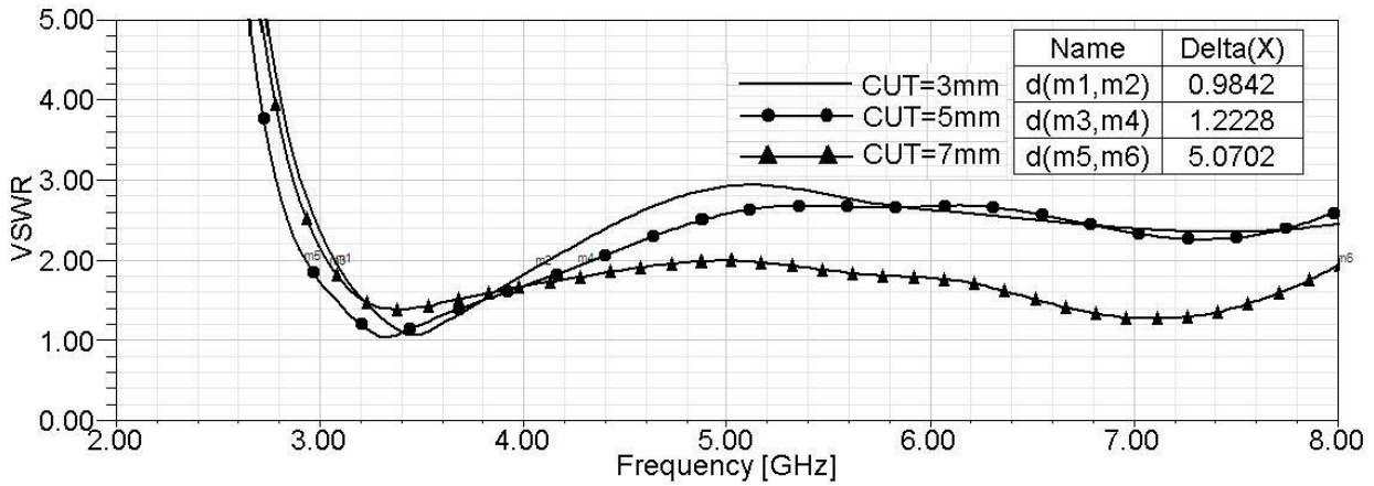
Figure 6. VSWR vs. Frequency for modified RMSA with straight edge cut
