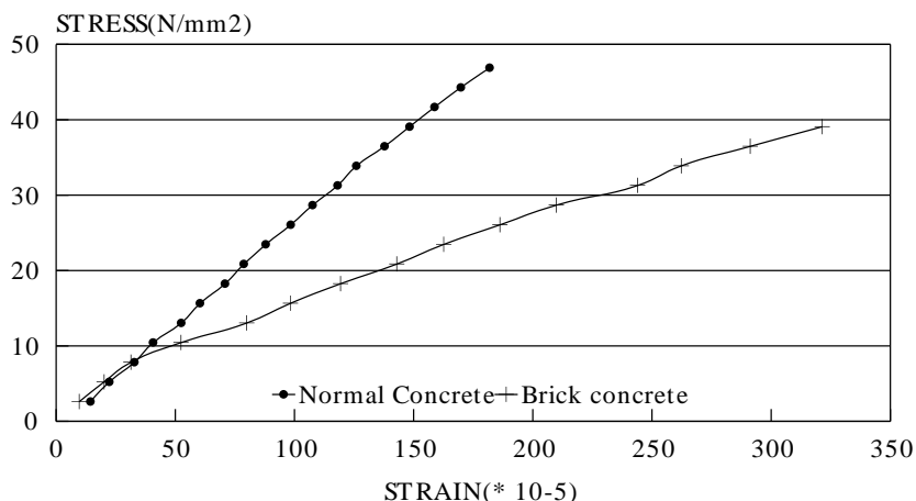
Figure 4. Stress/strain behaviour w/c ratio 0.24
