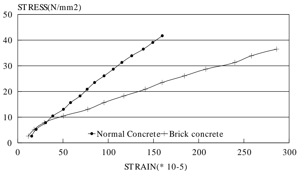
Figure 3. Stress/strain behaviour w/c ratio 0.29
