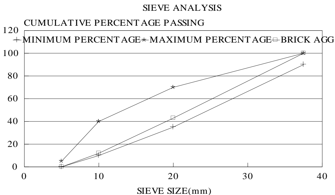
Figure 1. Sieve Analysis Minimum and maximum percentages given in BS 882.
