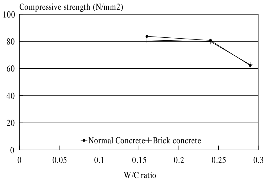
Figure 2. Compressive strength w/c ratio
