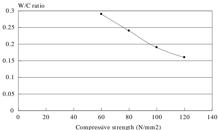
Figure 5. Design chart
