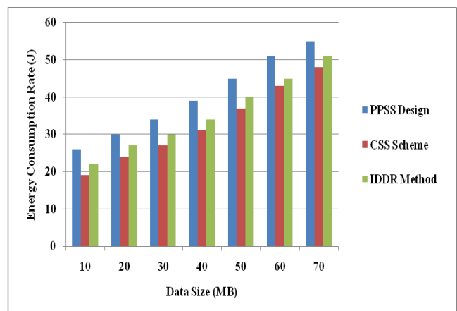
Figure 2. Energy Consumption Rate on Target Tracking and Data Collection in WSN
