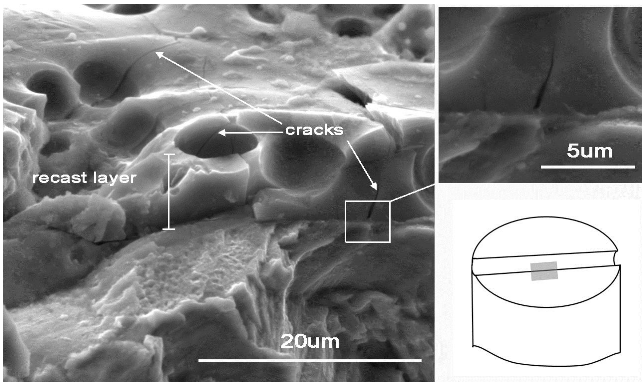
Figure 3. Rupture surface of a EDDHR specimen across the hole boundary. The grey rectangle in the scheme indicates the observation area.
