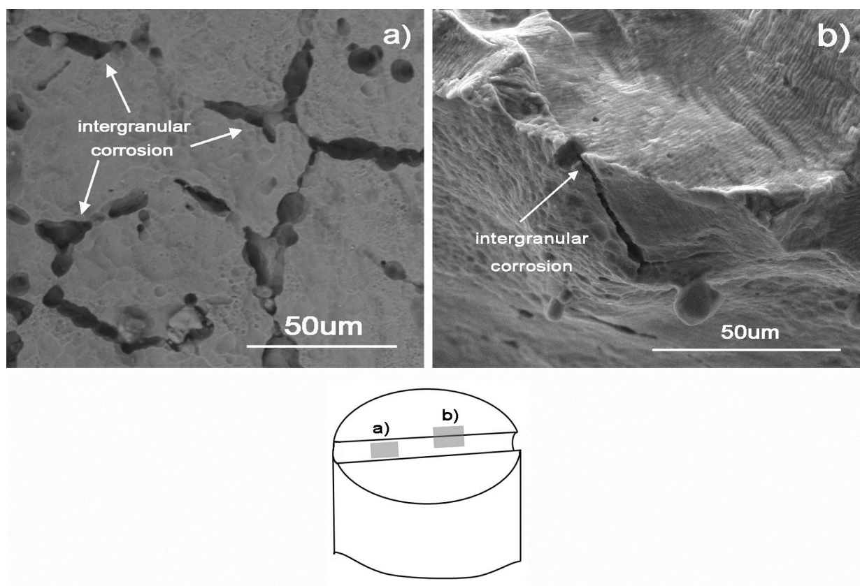
Figure 4. EDDL specimen: a) hole inner surface; b) hole boundary.
