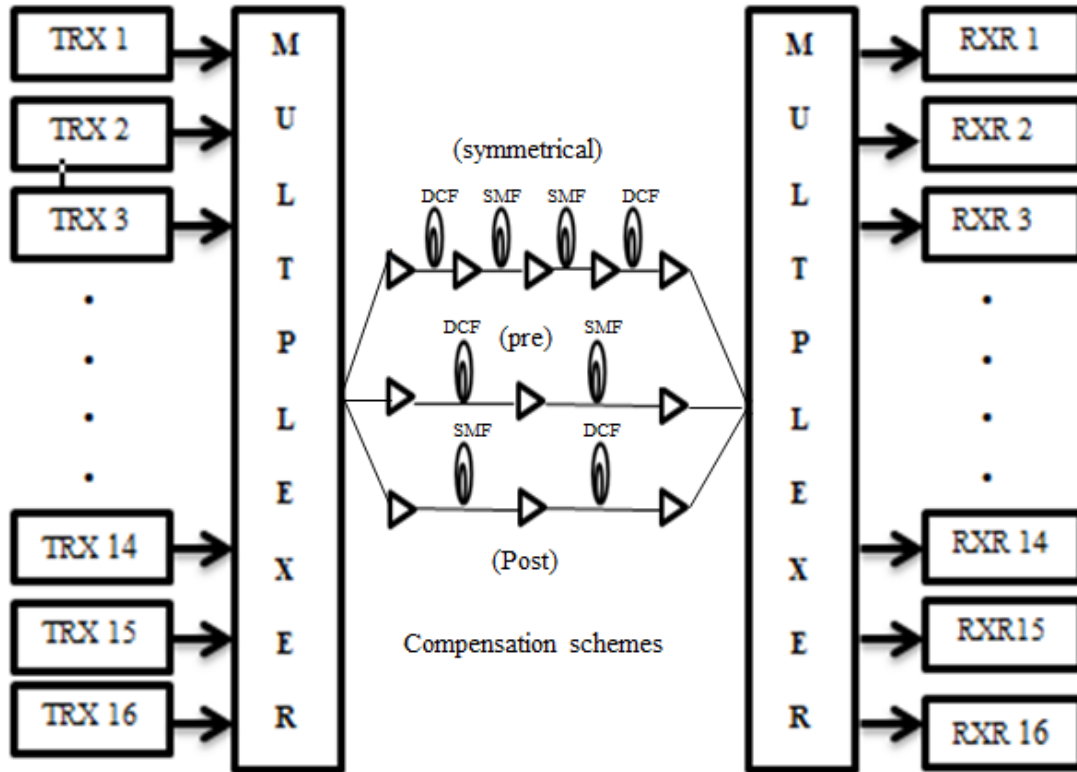
Figure 1. 16 channel DWDM System
