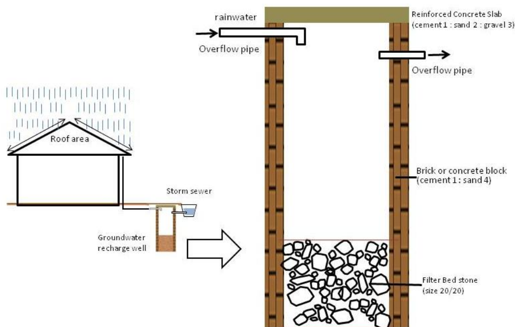
Figure 3. Schematic diagram of storm water recharge well facility and its design.
