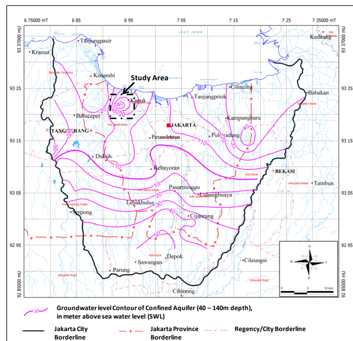
Figure 2. Map of Groundwater contour[14] and study area shown in dot-dashed square.
