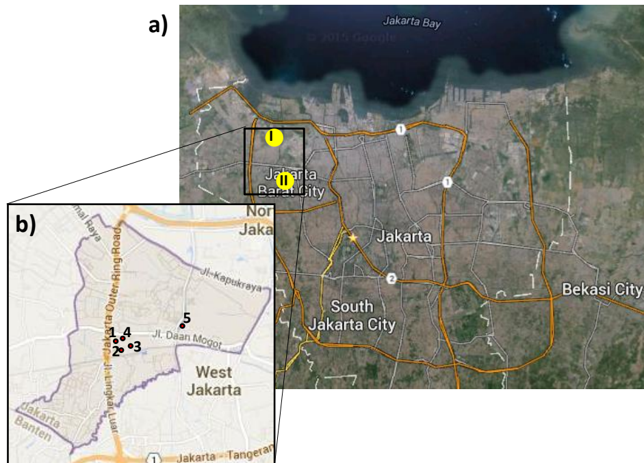
Figure 1. Sampling location of study of groundwater level (a) and groundwater quality (b) in Cengkareng Sub-district, West Jakarta Regency, Jakarta
