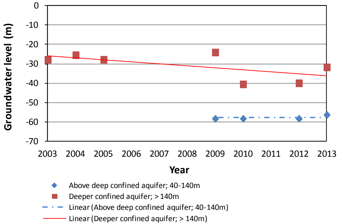
Figure 4. Groundwater level trend line of above confined aquifer (40 – 140 m) and deeper confined aquifer (>140m) (Source : Analysis Result 2014)
