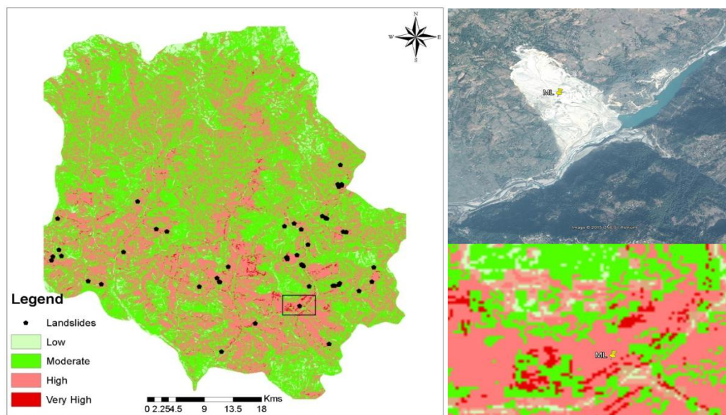
Fig. 4. Landslide Hazard map with Google Earth image of Sunkoshi Landslide event (ML represents massive landslide event)
