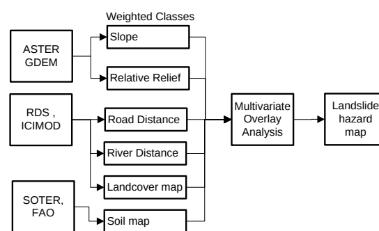
Fig. 3. Methodology of Landslide Hazard Zonation
