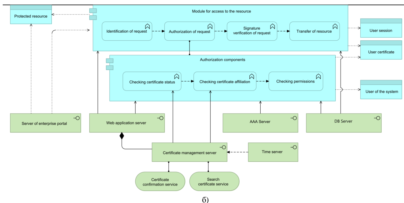
Figure 5 – Resource request authorization scheme: a – representation layer, б – application layer
