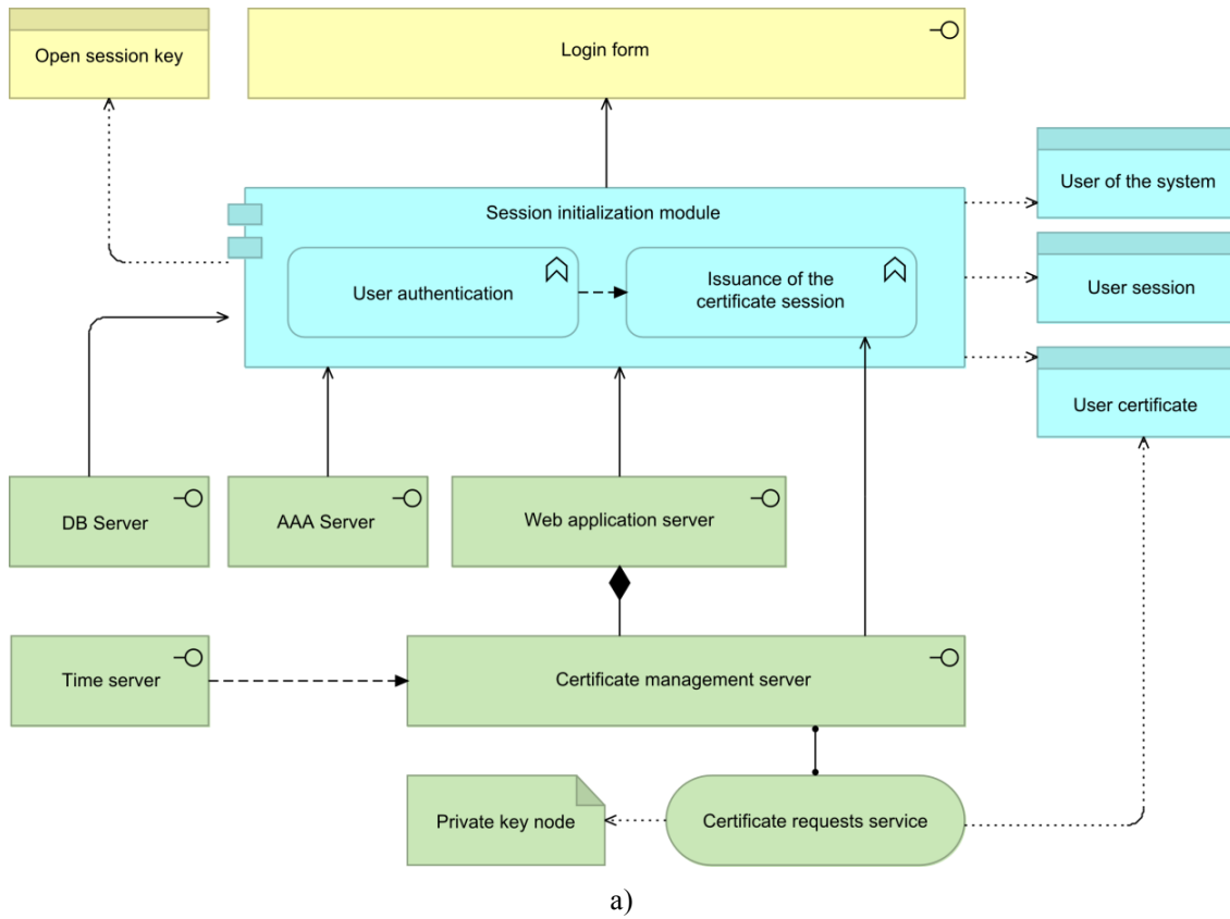
Figure 3 – Application layer schemes: a – administration components, б – registration components
