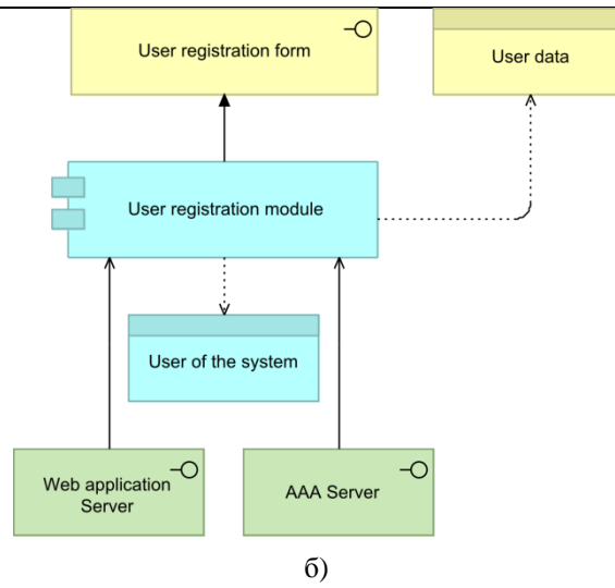
Figure 3 – Application layer schemes: a – administration components, б – registration components
