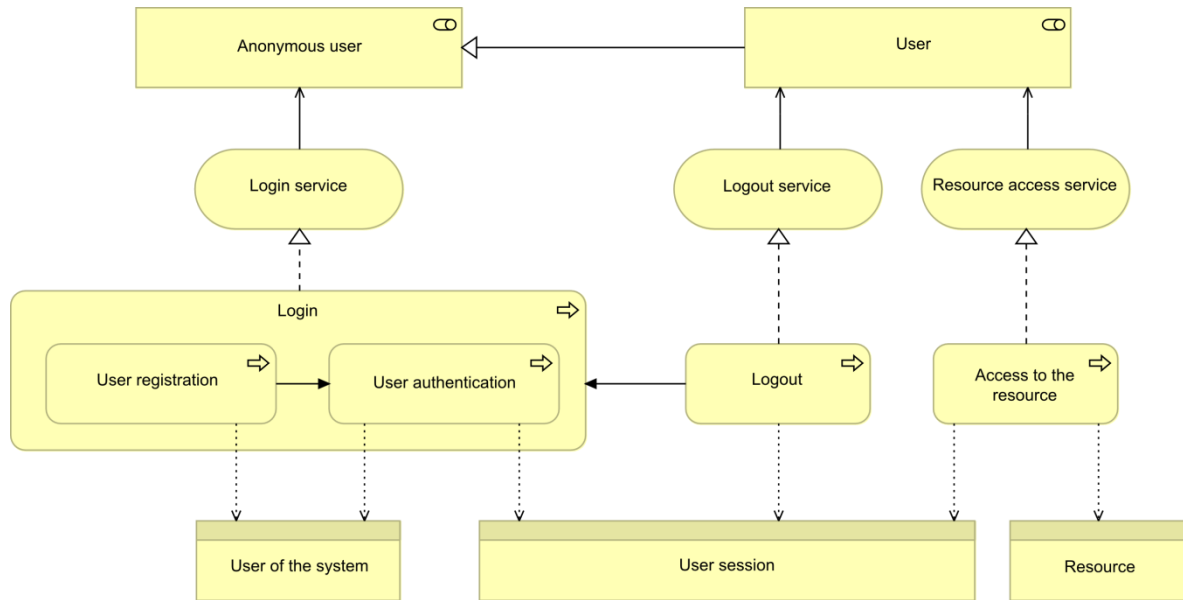
Figure 1 – General scheme of presentation layer
