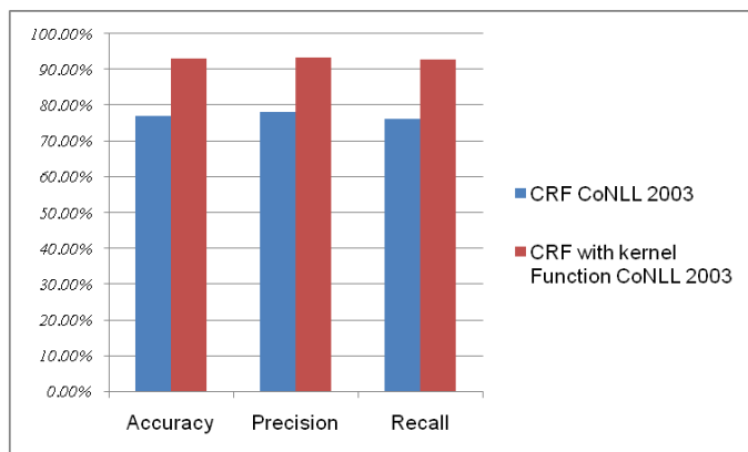
Figure 2. Diagrammatically representation of comparison between CRF and CRF with kernel function models for Entity Extraction
