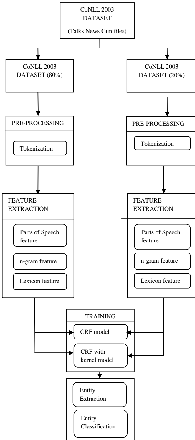
Figure 1. Proposed Methodology for Entity Extraction and Classification
