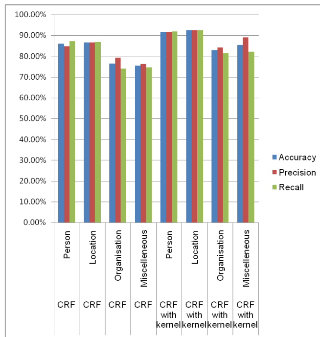
Figure 3. Diagrammatically representation of comparison between CRF and CRF with kernel function models for Entity Classification
