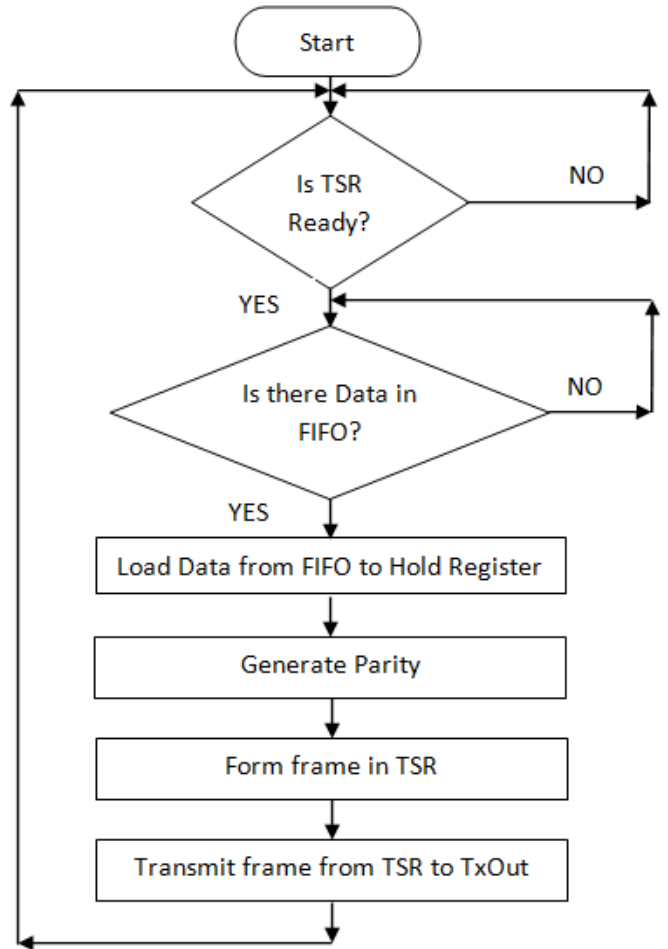
Fig. 5: Transmitter Flowchart – FIFO to TXOUT
