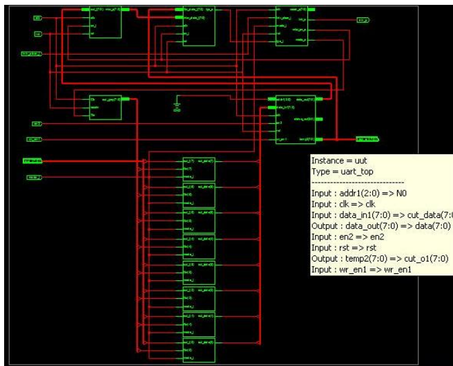
Fig. 11: RTL Schematic of UART with BIST
