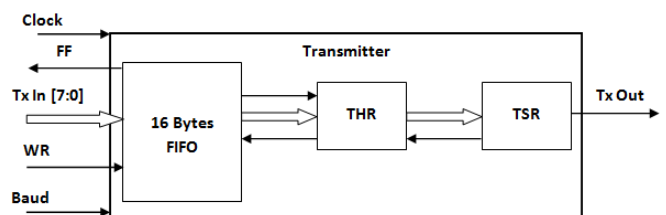
Fig. 3: UART Transmitter
