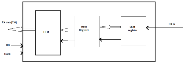
Fig. 7: UART Receiver
