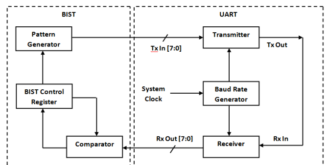
Fig. 2: UART with BIST Architecture
