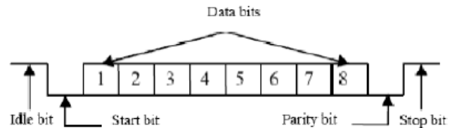
Fig. 6: UART Frame Format
