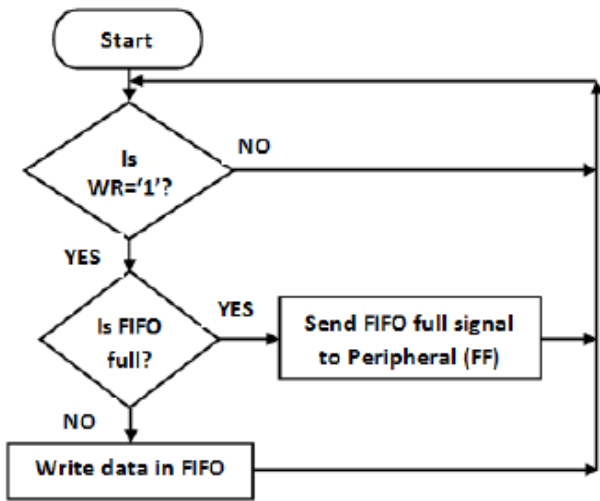
Fig. 4: Transmitter Flowchart – Input to FIFO
