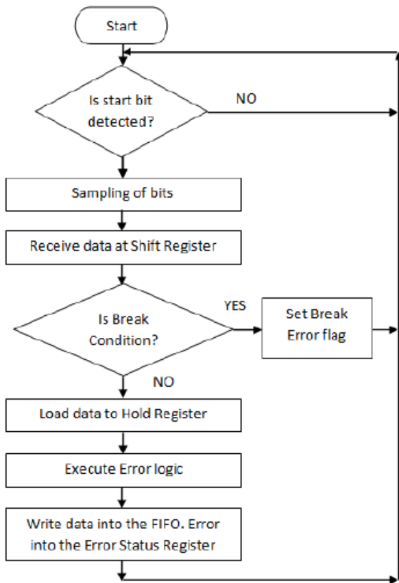
Fig. 8: Receiver flowchart (Input to FIFO)
