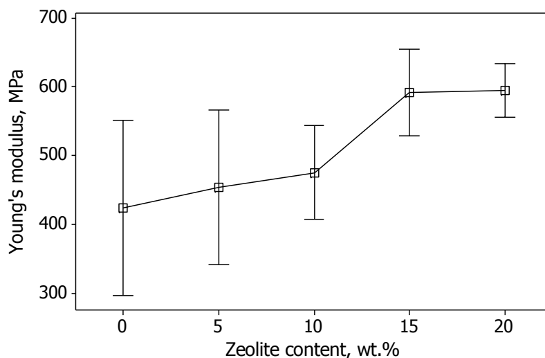
Figure 6: Young's Modulus As A Function of Zeolite Content
