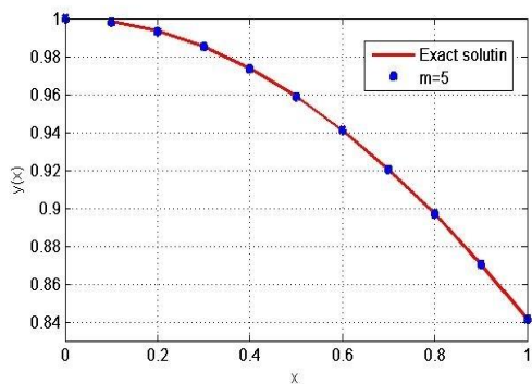
Figure 2: Graph of exact solution and approximate solution at m=5
