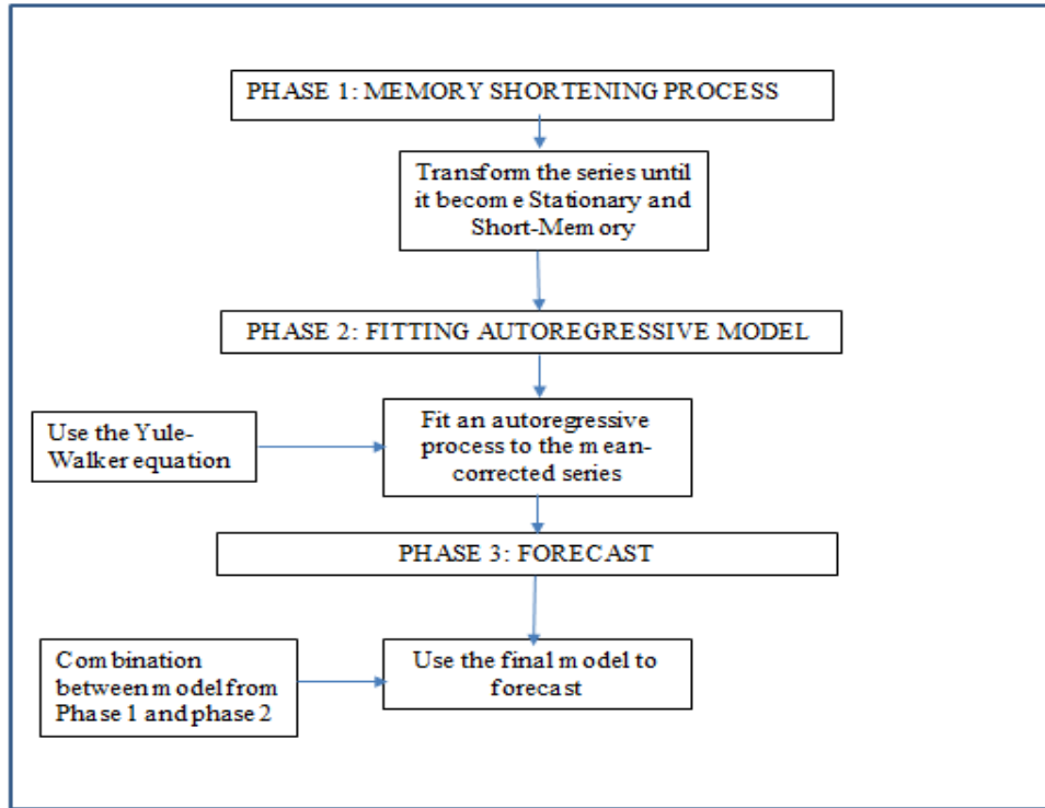
Figure 1: ARAR Algorithm process
