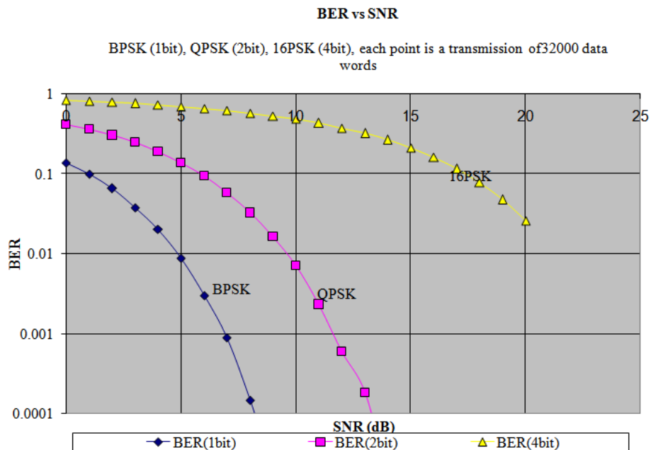
Figure 5: Graph between BER VS SNR.
