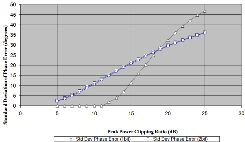
Figure 4: Graph between Standard Deviation Of Phase Error Vs Peak Power Compression Due To Clipping.
