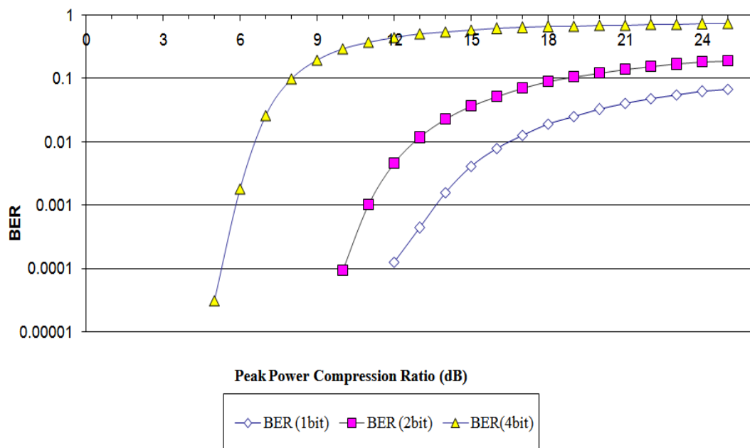
Figure 3: Graph Between BER Vs Peak Power Compression Due To Clipping.
