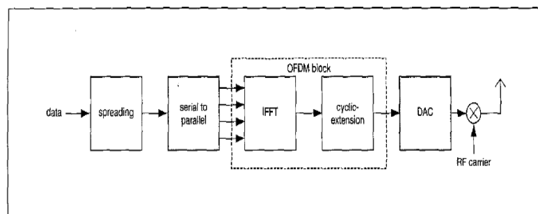
Figure 1: Transmitter of MC CDMA.
