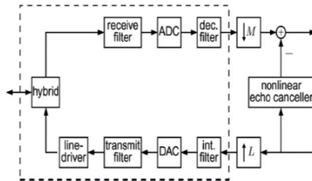
Fig. 2: Echo path in a full-duplex communication system.
