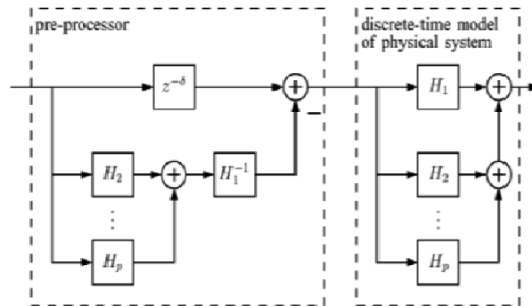
Fig. 1: Linearization of a weakly nonlinear system modelled as a p th-order Volterra filter using a pre-processor.
