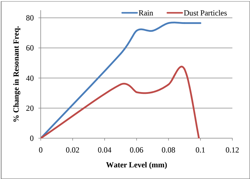
Fig. 3: Percentage change in the resonant frequency versus height of superstrate layers on the microstrip patch surface.
