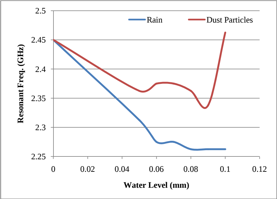
Fig. 2: Resonant frequency versus height of superstrate layers over the microstrip patch surface.
