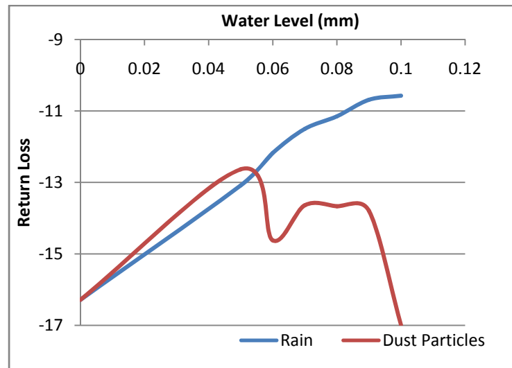
Fig. 4: Return loss versus height of superstrate layers on the microstrip patch surface.
