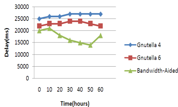
Plot 2: Query Delay
