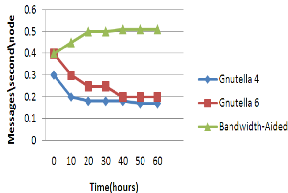
Plot 1: Maintenance Overhead.
