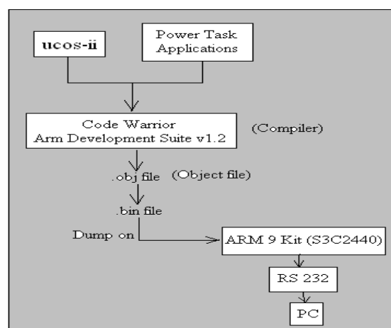
Figure 4: Complete Project Process Flow.
