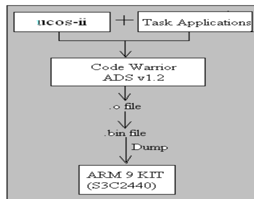
Figure 3: Project process flow (Software approach).
