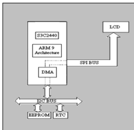
Figure 2: Execution of applications through DMA (Direct Memory Access) without CPU intervention.
