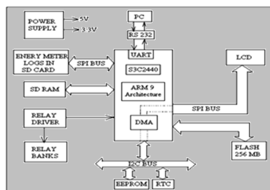
Figure 1: Block diagram of Priority dynamic scheduler for power Applications through DMA Peripherals
