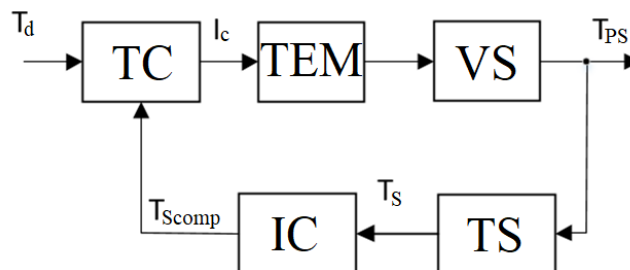
Figure 2 - Block diagram of the climate control system based on Peltier thermoelectric modules
