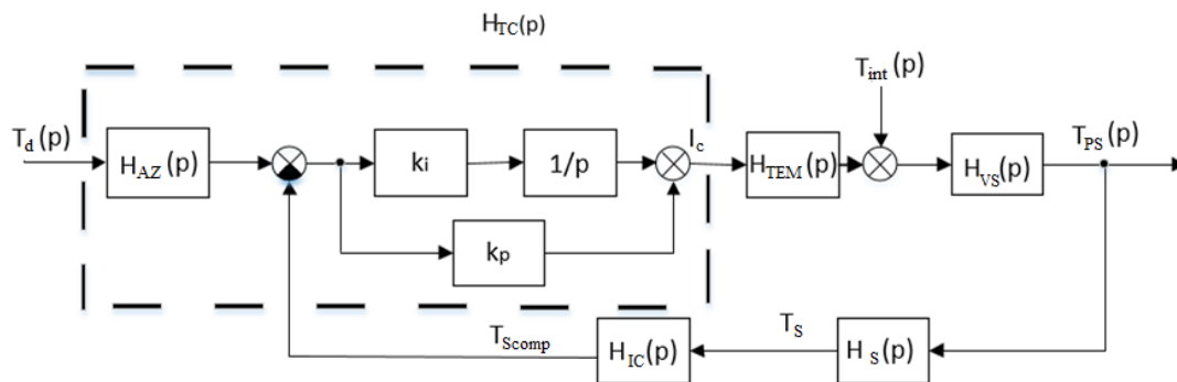
Figure 3 - Equivalent functional model of the climate control system based on Peltier thermoelectric modules
