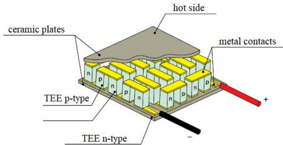
Figure 1 - The structure of the thermoelectric module based on the Peltier effect
