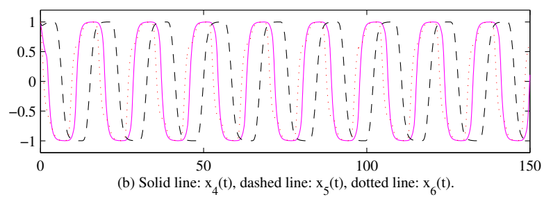
Figure 4.2: Periodic oscillation of the solutions, delays:
