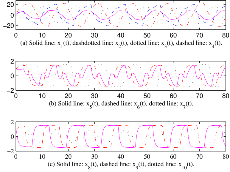
Figure 4.6: Periodic oscillation of the solutions, delays:
