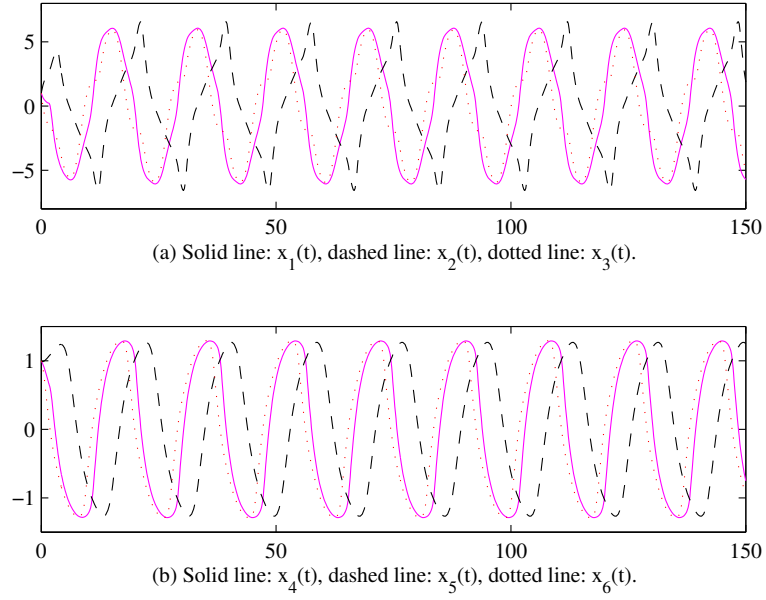
Figure 4.3: Periodic oscillation of the solutions, delays:
