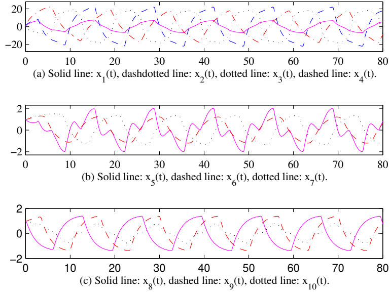
Figure 4.5: Periodic oscillation of the solutions, delays:
