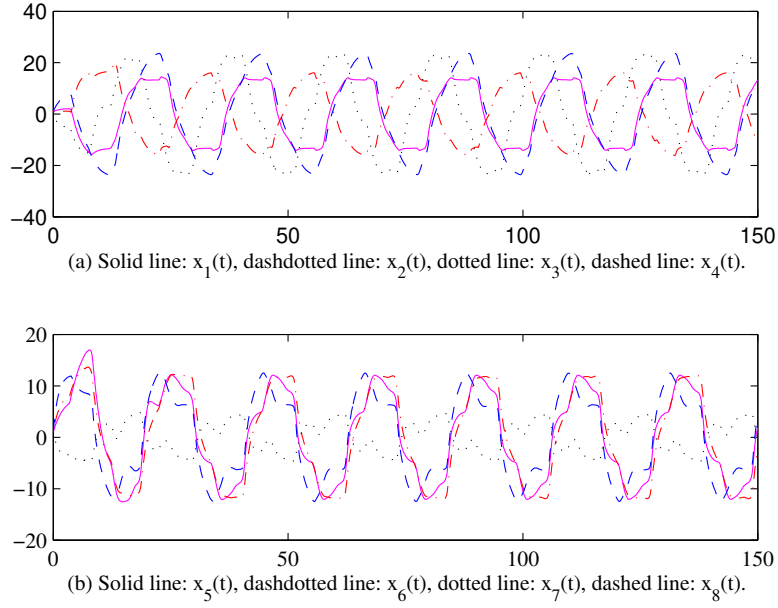
Figure 4.9: Periodic oscillation of the solutions, delays:
