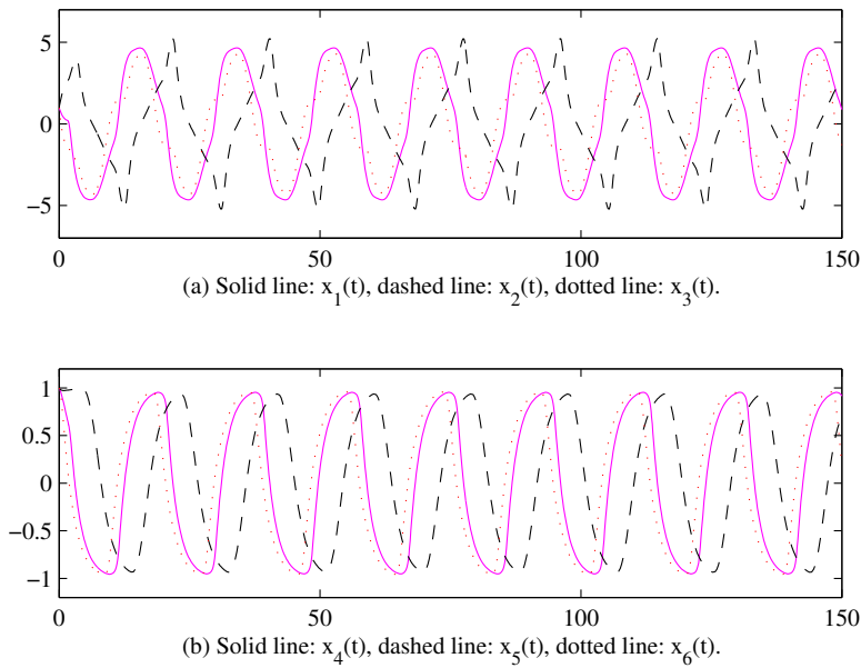
Figure 4.1: Periodic oscillation of the solutions, delays:
