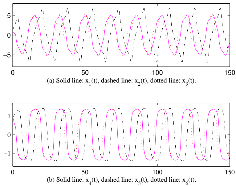
Figure 4.4: Periodic oscillation of the solutions, delays:
