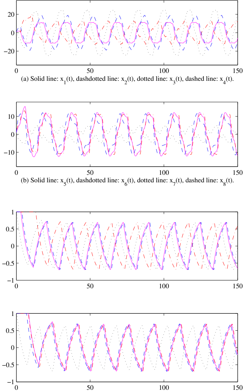
Figure 4.7: Periodic oscillation of the solutions, delays:
