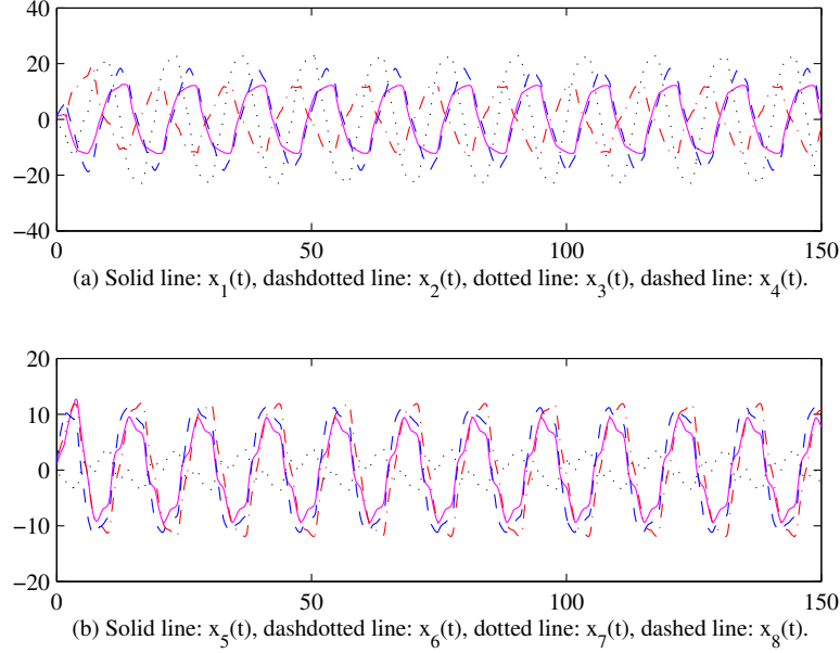
Figure 4.10: Periodic oscillation of the solutions, delays:
