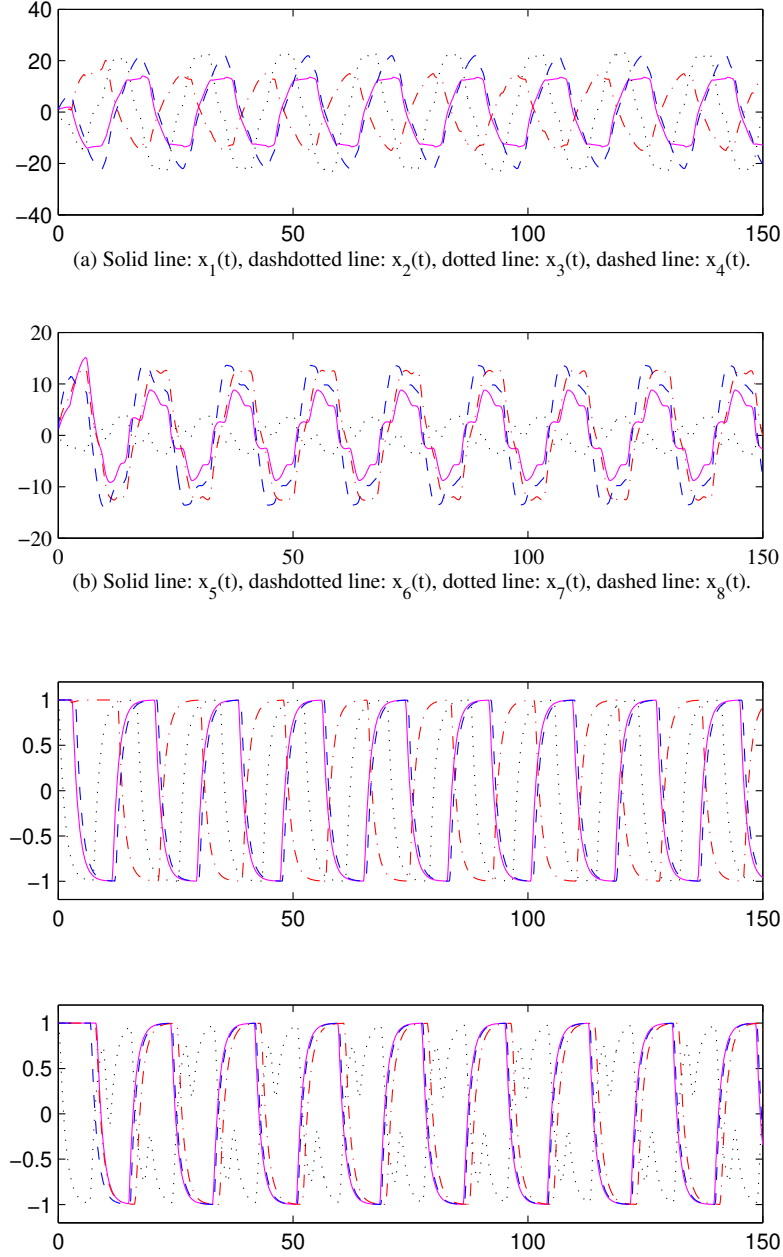
Figure 4.8: Periodic oscillation of the solutions, delays:
