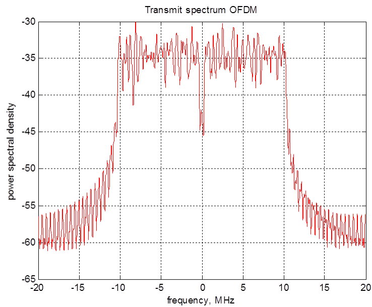
Fig.6: Spectrum of OFDM signal
