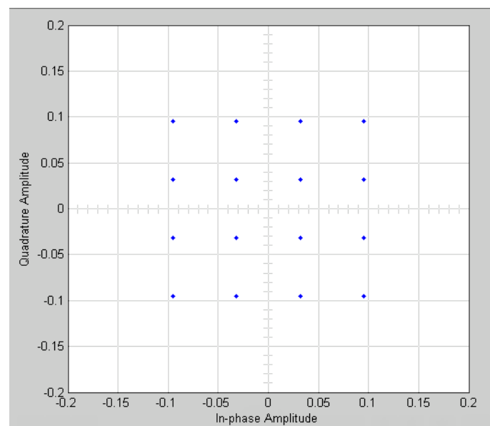
Fig. 11: Signal constellation diagram
