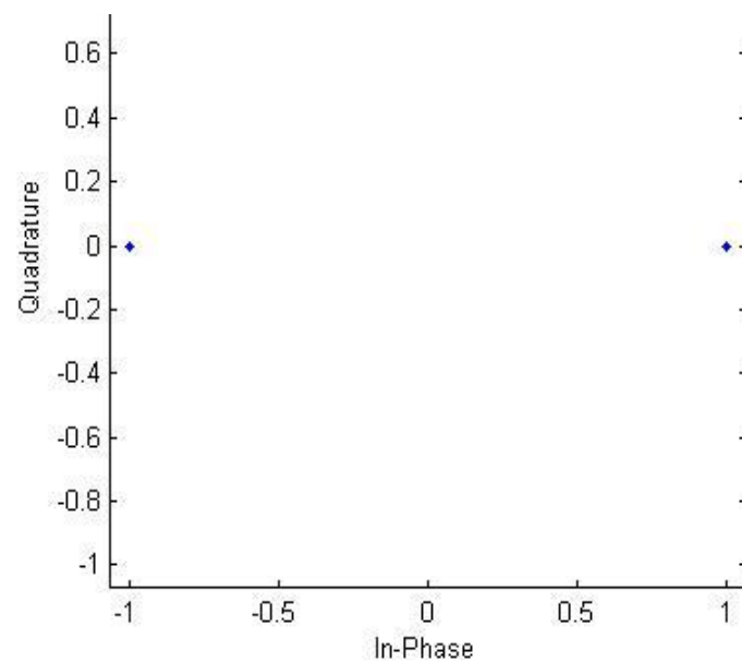
Fig7: Signal constellation diagram
