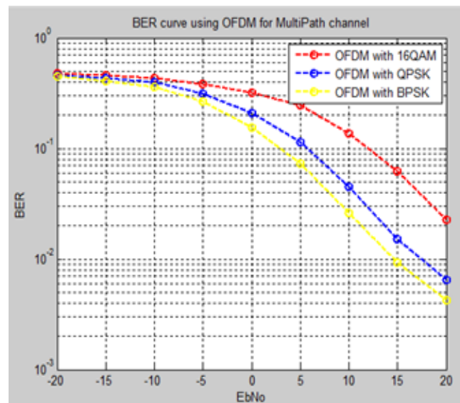
Fig.13: BER curves
