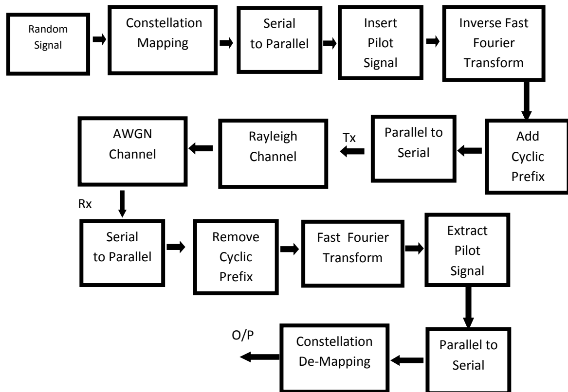
Fig.4 OFDM Simulation Model
