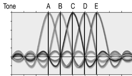
Fig.2 Tones for OFDM
