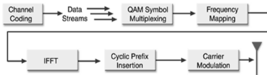
Fig. 3 OFDM transmitter chain
